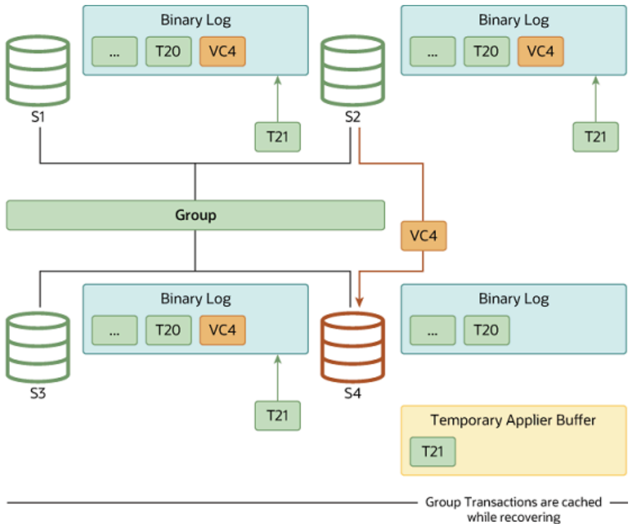
Figure 17.13 Queued Transactions
