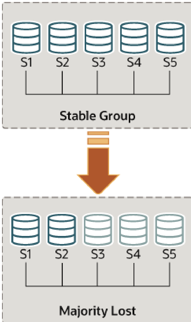
Figure 17.7 Losing Quorum
