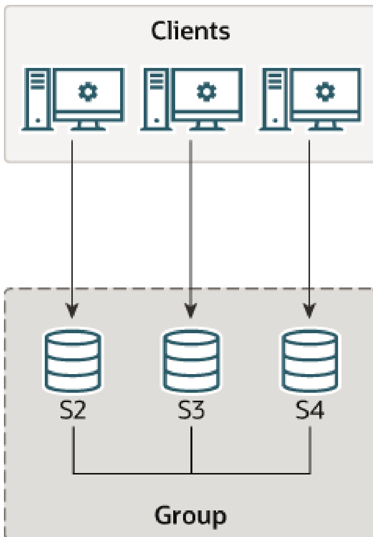
Figure 17.4 Group Architecture
