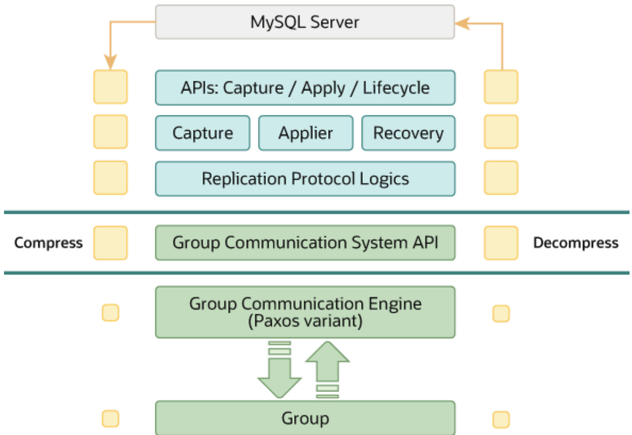
Figure 17.15 Compression Support
