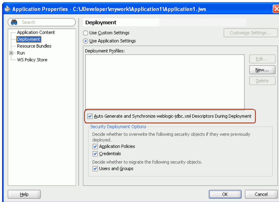
Figure 64–5 Auto Generate and Synchronize weblogic-jdbc.xml Descriptors During Deployment Checkbox
