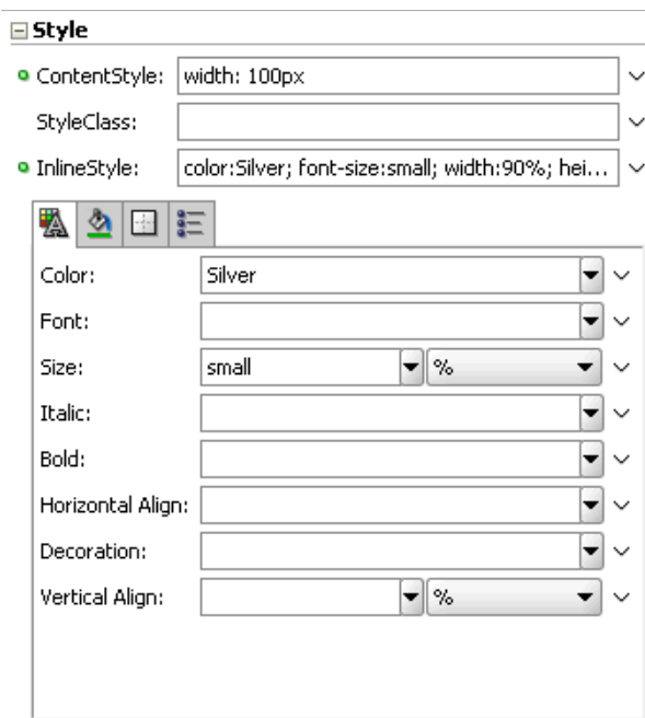
Figure 21–10 Defining Styles for contentStyle and inlineStyle in the Property Inspector
