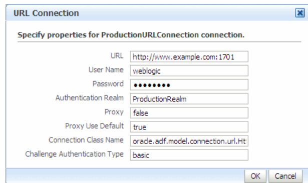
Figure 9–8 URL Connection Dialog
