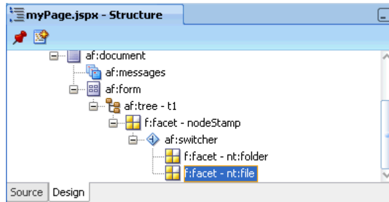
Figure 27–35 Switcher Component with Two Facets
