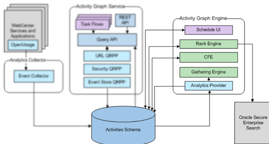
Figure 41–3 Data Gathering by the Activity Graph Engine
