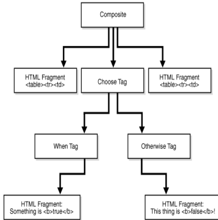
Figure 58–5 Tag Transformation Engine Tree
