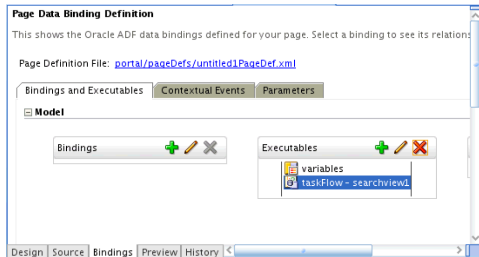
Figure 40–3 Page Data Binding Definition
