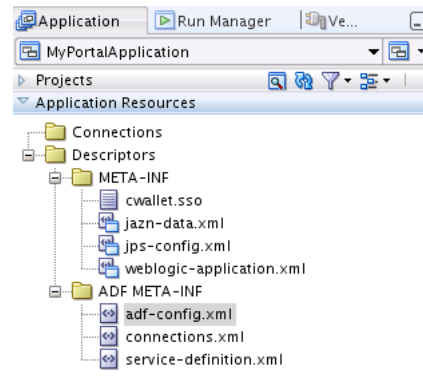
Figure 8–16 Location of the adf-config.xml File in JDeveloper
