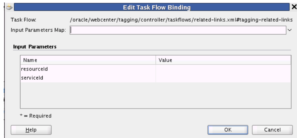
Figure 39–6 Edit Task Flow Binding Dialog for Tags - Related Links Task Flow
