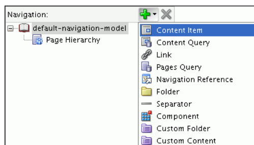
Figure 10-3 The Add New Node Menu
