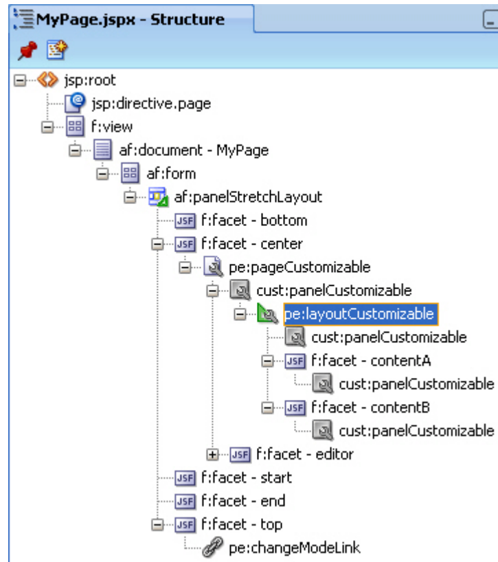
Figure 19–5 Layout Customizable Component
