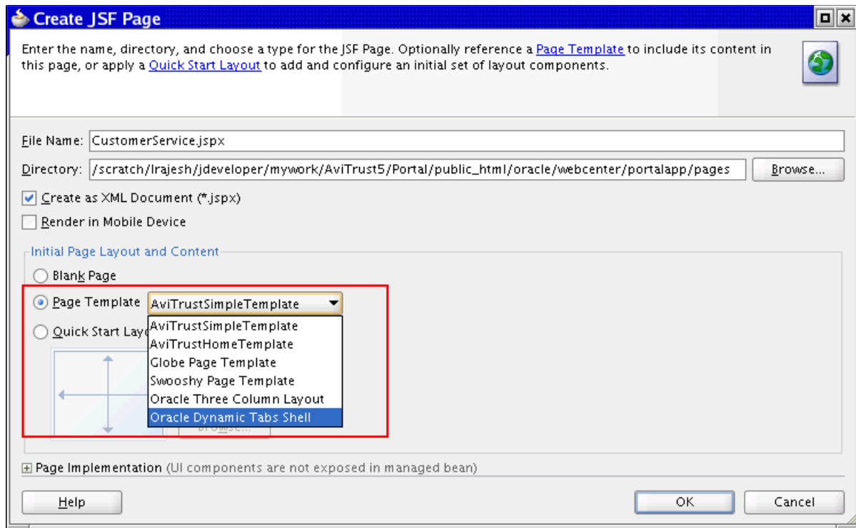
Figure 11–2 Page Template Option in the Create JSF Page Dialog
