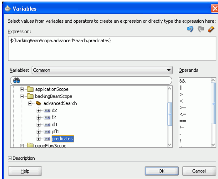
Figure 27–40 Variables Dialog - predicates
