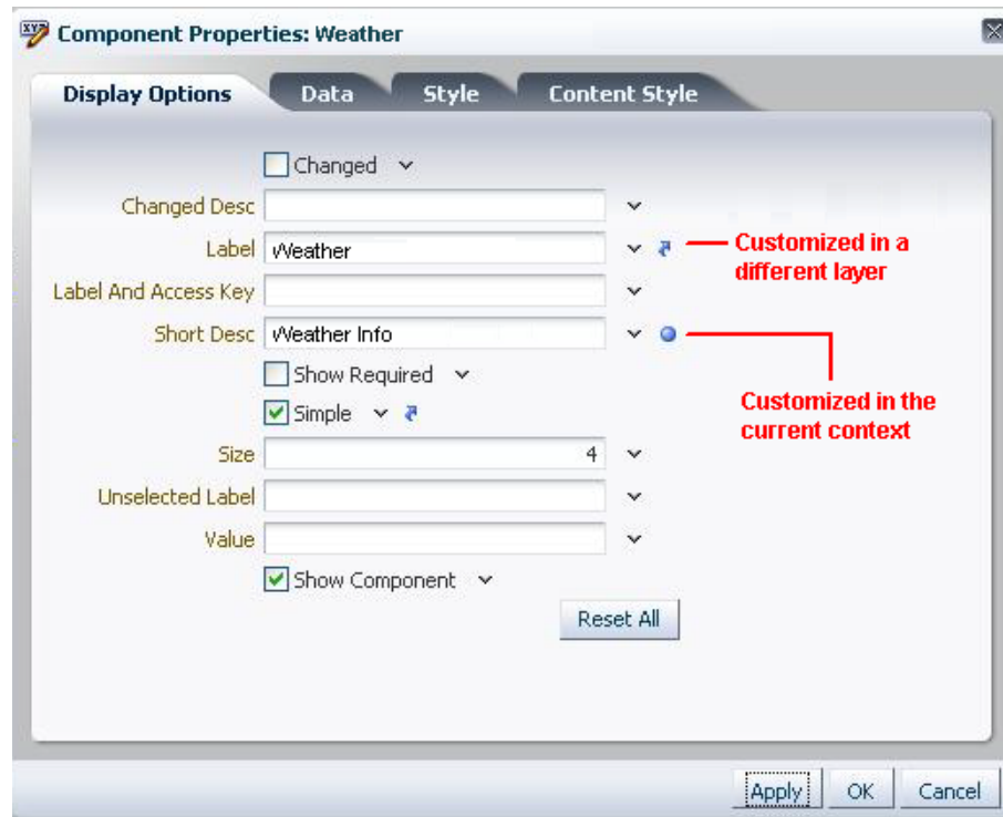
Figure 17–26 Visual Indication of Property Customization
