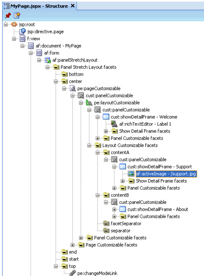
Figure 19–8 Component Hierarchy in MyPage.JSPX
