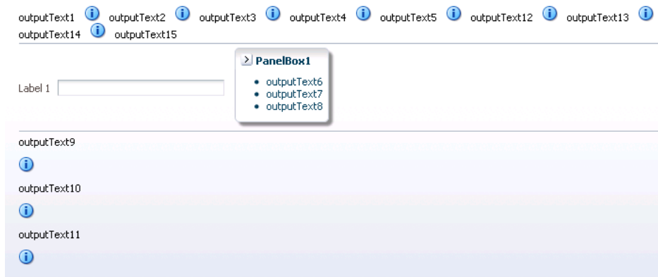
Figure 8–49 panelGroupLayout Arrangements
