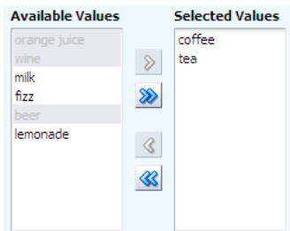
Figure 9–26 selectManyShuttle component
