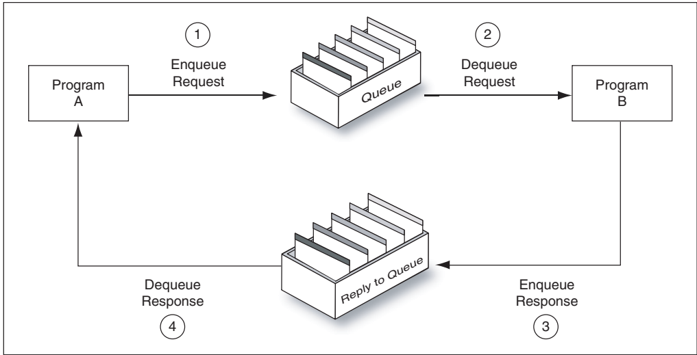
Figure 10-2 Request/Response Interaction
