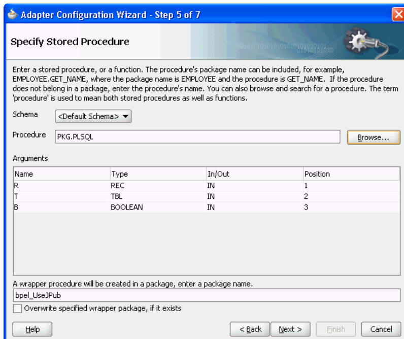
Figure 9–56 Specifying a Stored Procedure in the Adapter Configuration Wizard
