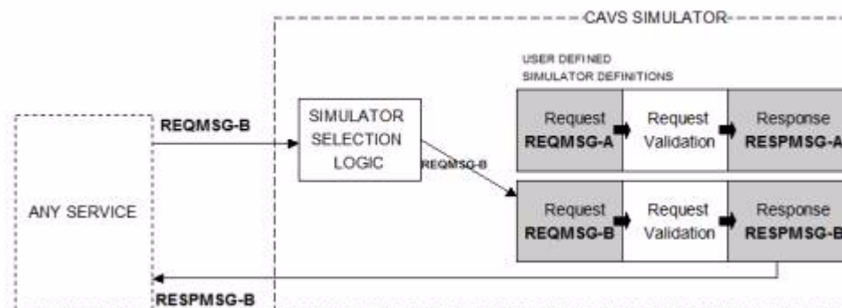
Figure 1–2 CAVS Simulator
