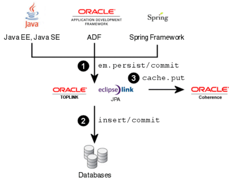
Figure 2–3 Writing and Persisting Objects in grid Cache Configuration
