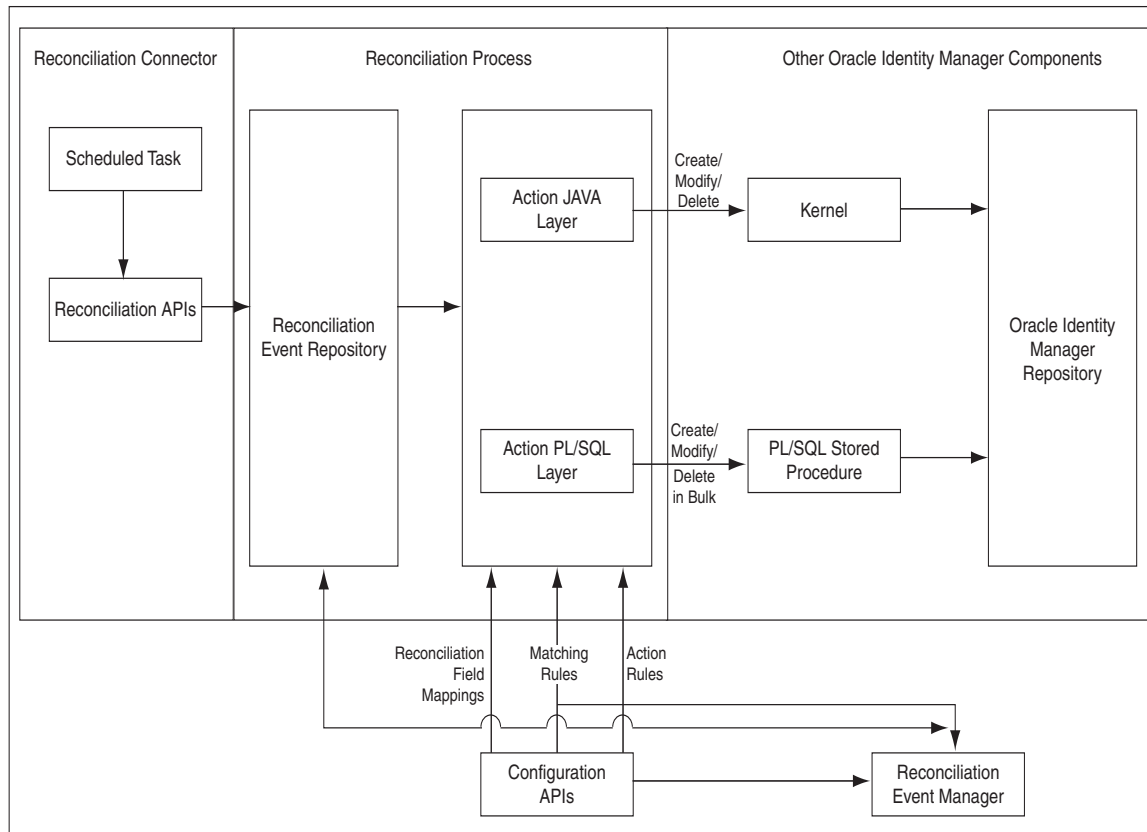
Figure 4-7 Reconciliation Architecture
