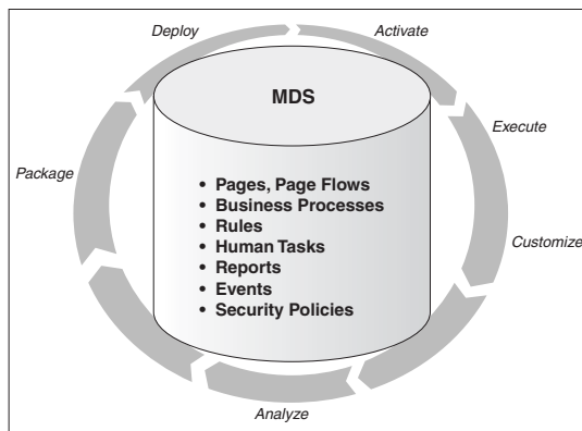
Figure 2–5 Metadata Services
