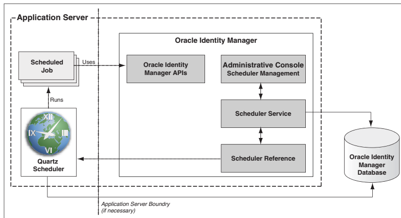
Figure 2–4 Oracle Identity Manager Scheduler Architecture
