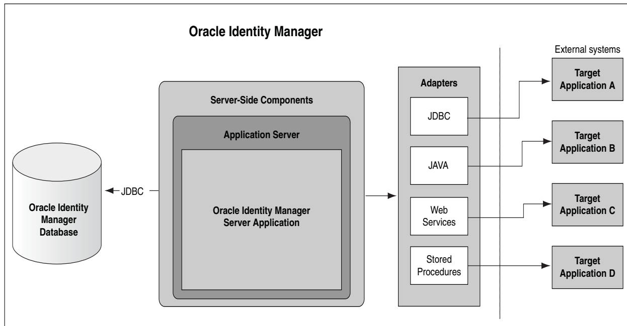
Figure 4–1 Provisioning Configuration
