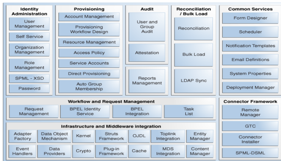
Figure 2–6 System Components of Oracle Identity Manager
