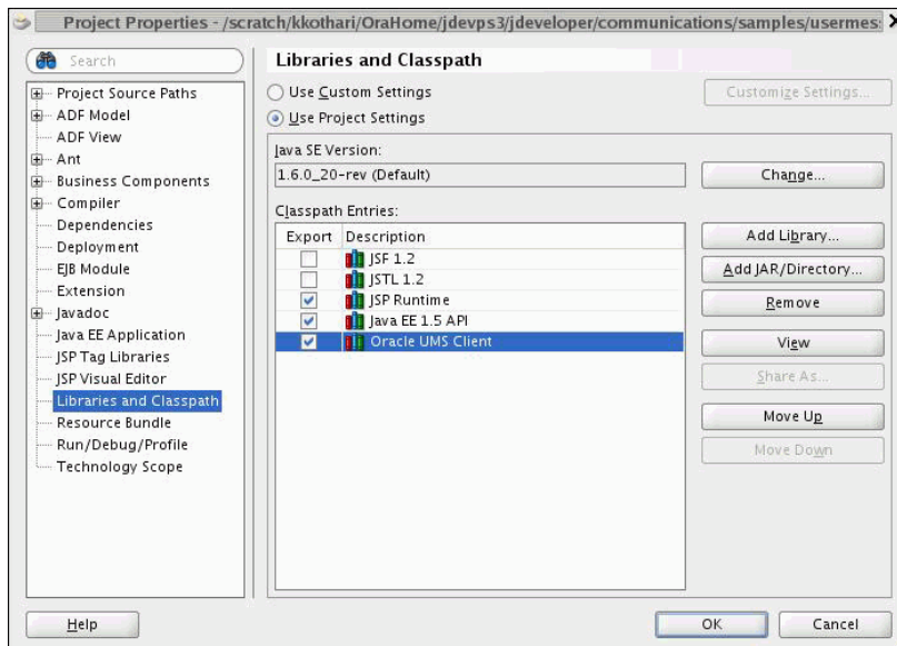
Figure 60–2 Verifying Libraries
