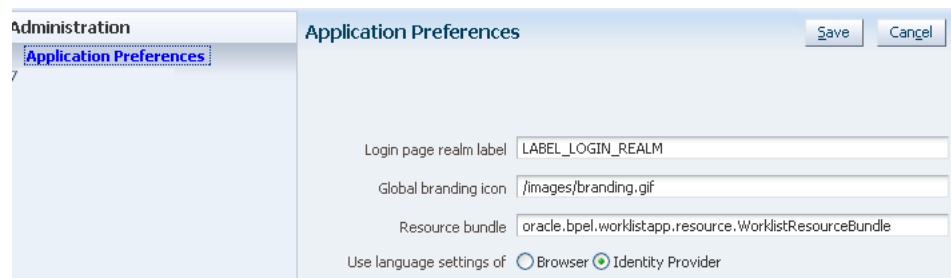
Figure 30-66 Application Preferences
