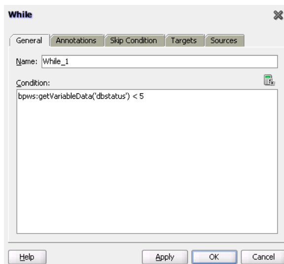
Figure A–47 While Dialog
