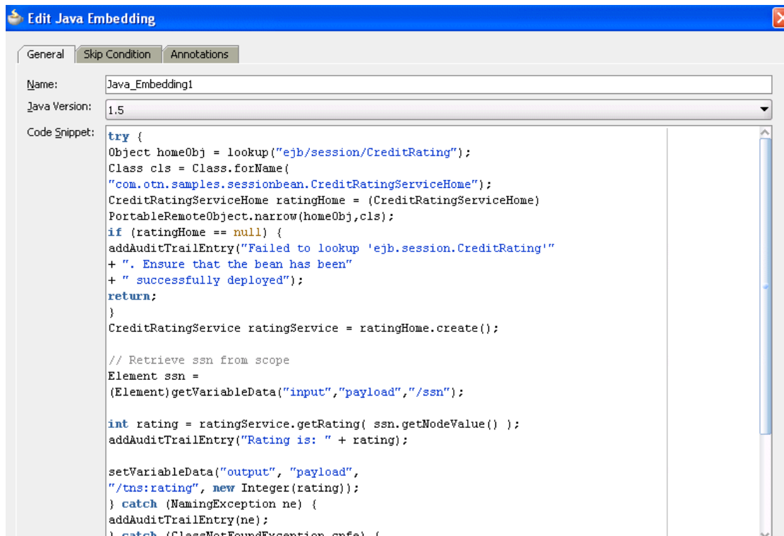
Figure A–21 Edit Java Embedding Dialog
