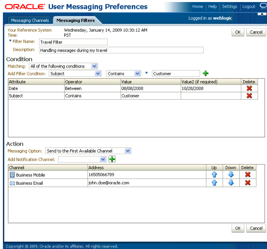
Figure 64–9 Creating a Filter
