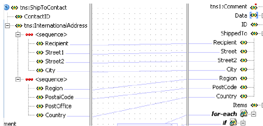
Figure 38–54 XSLT Mapper
