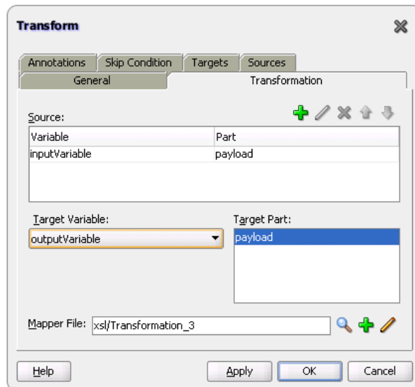
Figure 38–5 Transform Dialog
