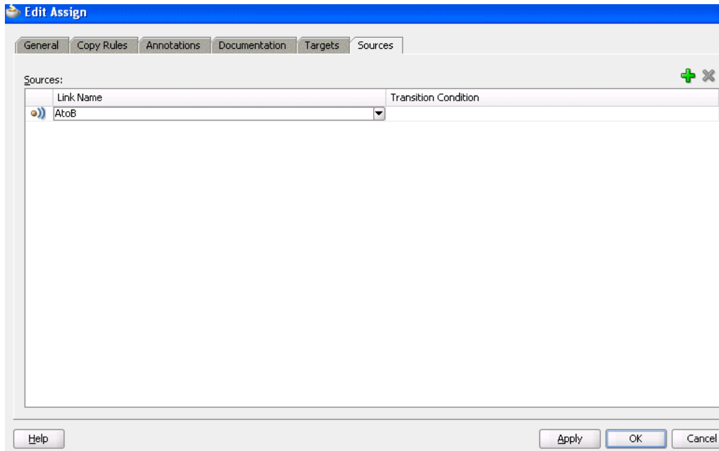
Figure 9–6 Source Activity
