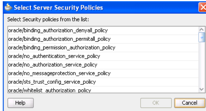
Figure 40–2 Security Policies
