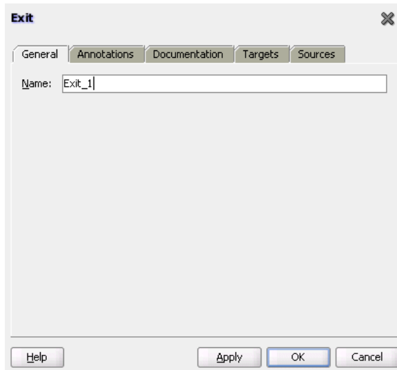
Figure 11-18 Exit Activity
