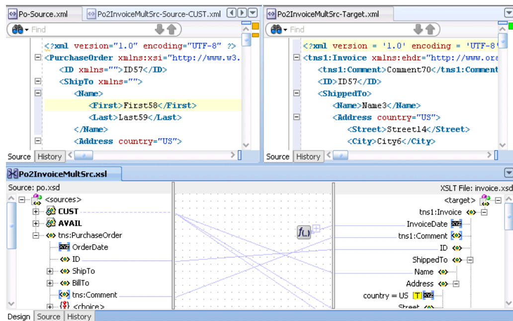
Figure 38–49 Test Results
