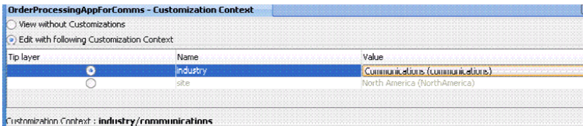
Figure 16-3 Customization Context
