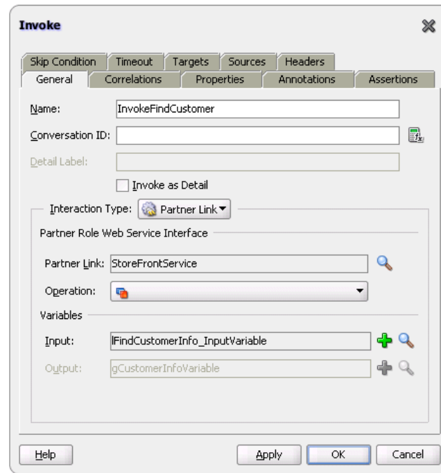
Figure 4–7 Invoke Activity Example
