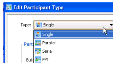
Figure 28–25 Type List
