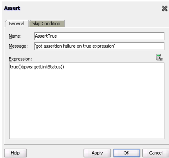
Figure 11–22 Assert Dialog
