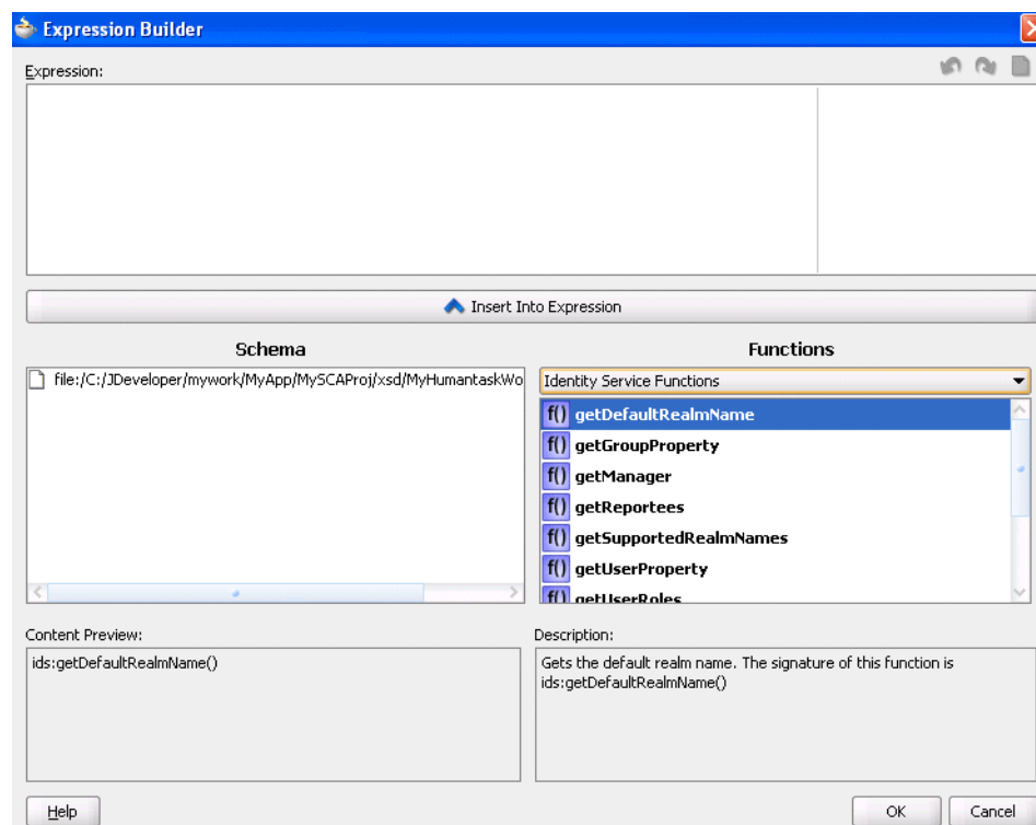
Figure 28–16 Expression Builder
