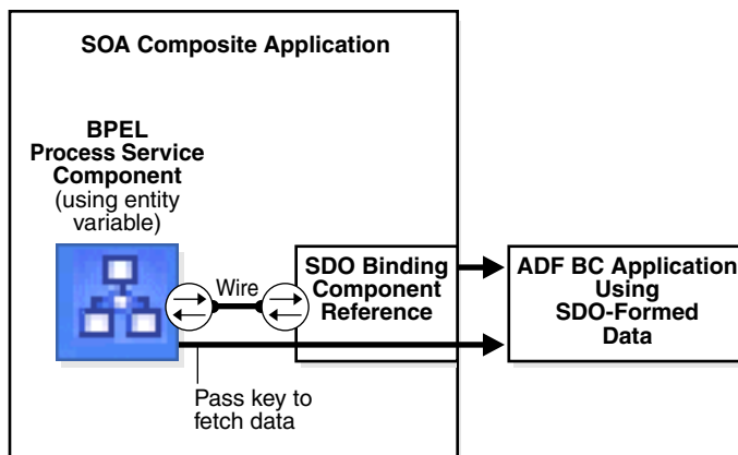
Figure 6–2 Outbound Direction
