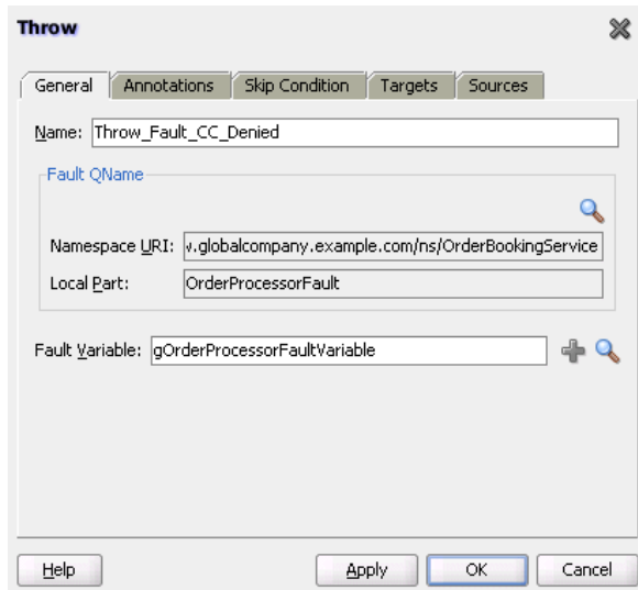
Figure 11–3 Throw Dialog
