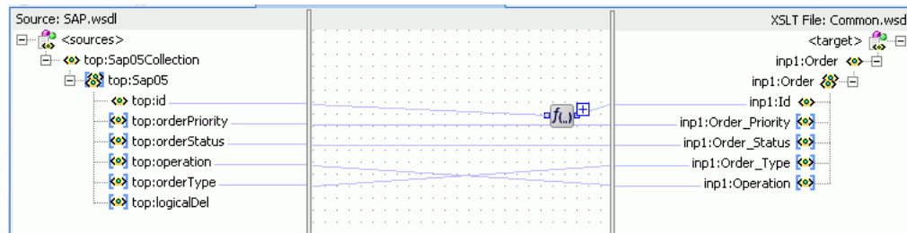
Figure 46–54 SAP_TO_COMMON_INSERT.xsl Transformation
