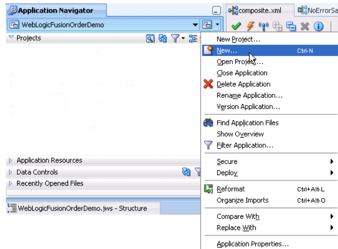
Figure 3–5 Application Menu
