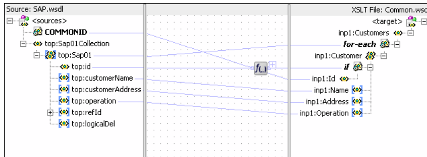
Figure 46–33 SAP_TO_COMMON_DELETE.xsl
