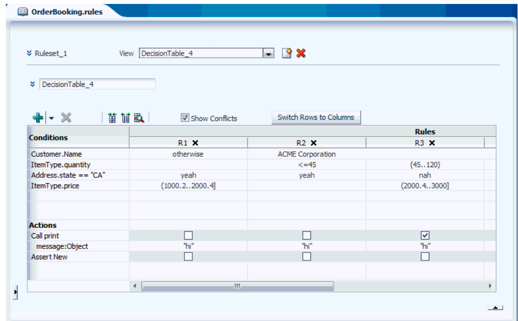
Figure 26–4 Decision Tables
