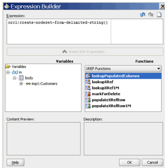
Figure 46–6 Expression Builder Dialog with Cross Reference Functions
