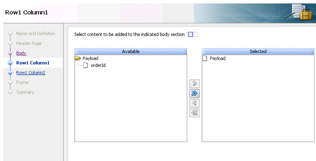
Figure 29–12 Custom Task Form Wizard: Selecting the Body Fields
