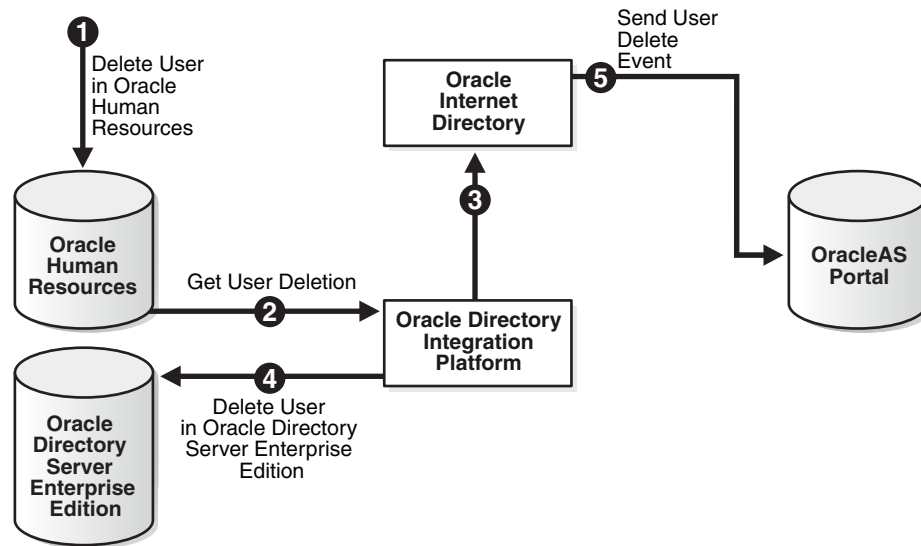
Figure D-4 Deletion of Users from the Corporate Human Resources
