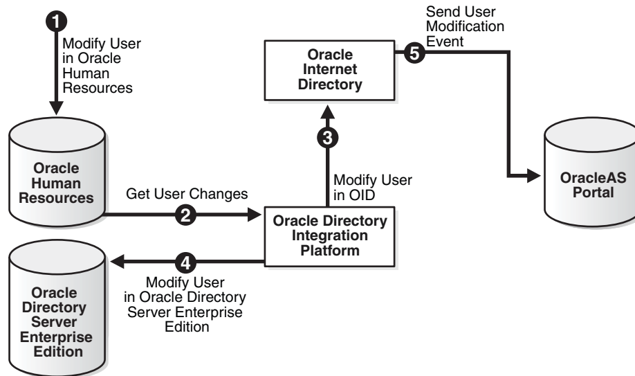
Figure D-3 Modification of User Properties
