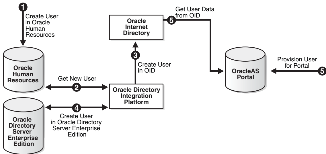
Figure D–2 User Creation and Provisioning
