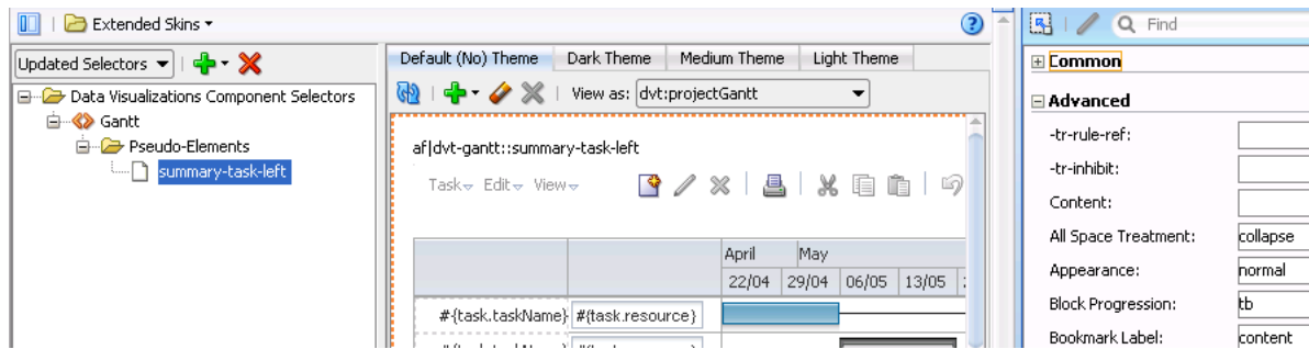
Figure 5-7 Properties for the gant Component summary-task-left Pseudo-Element
