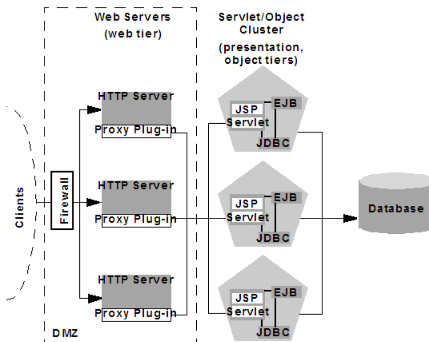
Figure 9-4 Two-Tier Proxy Architecture
