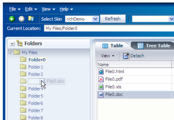
Figure 32–3 Drag and Drop Functionality in the File Explorer Application
