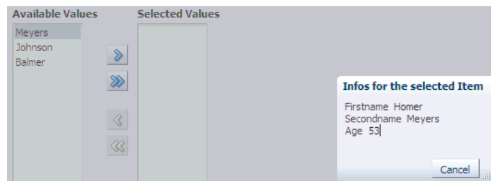
Figure 9–28 selectManyShuttle with selectionListener
