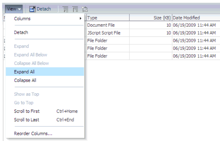
Figure 10–20 Panel Collection for Tree Table with Menu and Toolbar
