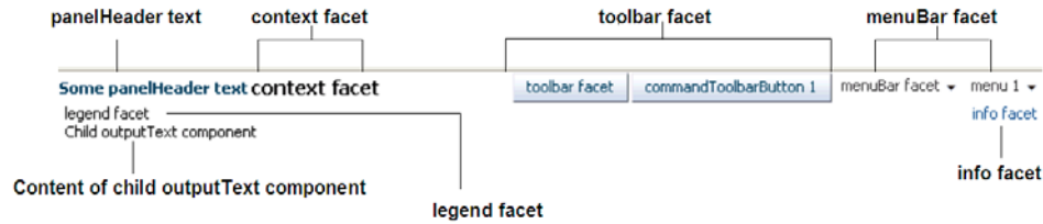
Figure 8–38 panelHeader and Its Facets
