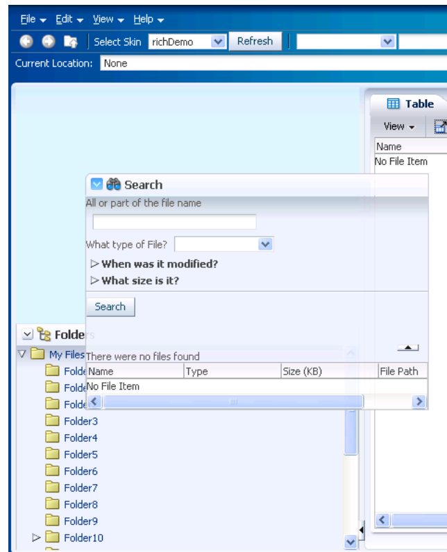
Figure 8-35 Panes Can Be Reordered by Dragging and Dropping
