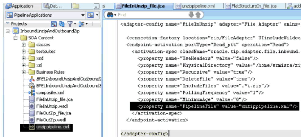
Figure 4–5 Project with unzippipeline.xml File
