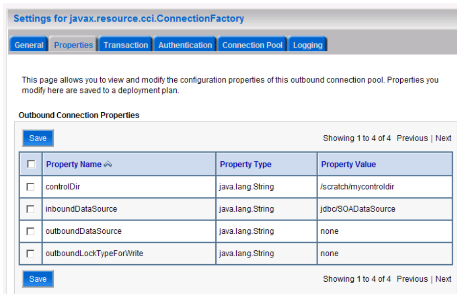
Figure 4–42 Oracle WebLogic Server Administration Console - Settings for javax.resource.cci.ConnectionFactory Page
