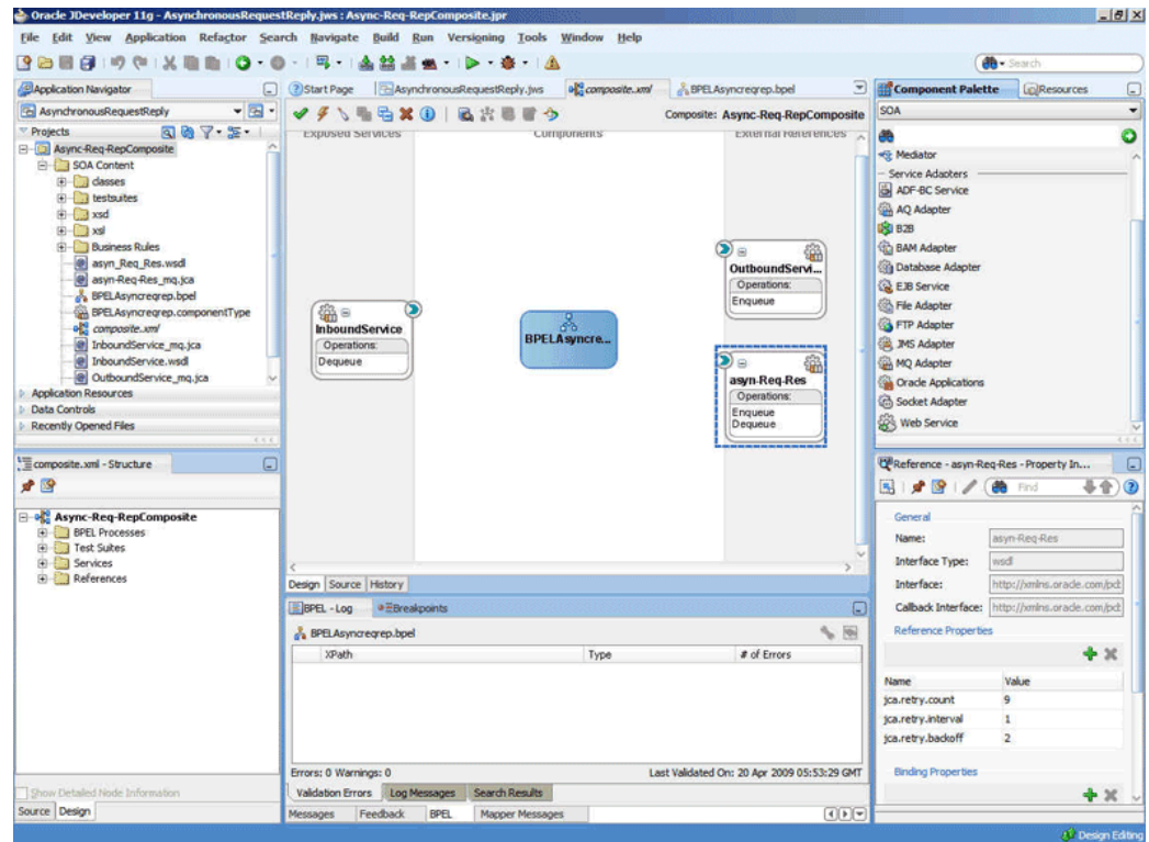
Figure 10-76 The JDeveloper Page - Composite.xml Page
