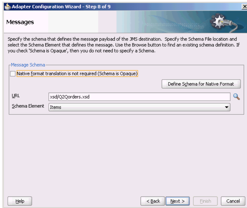
Figure 8–19 The Adapter Configuration Wizard - Message Page
