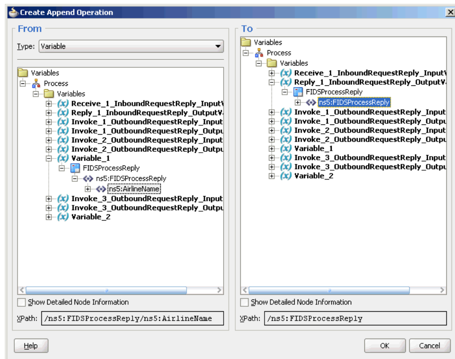
Figure 5–108 The Create Append Operation Dialog
