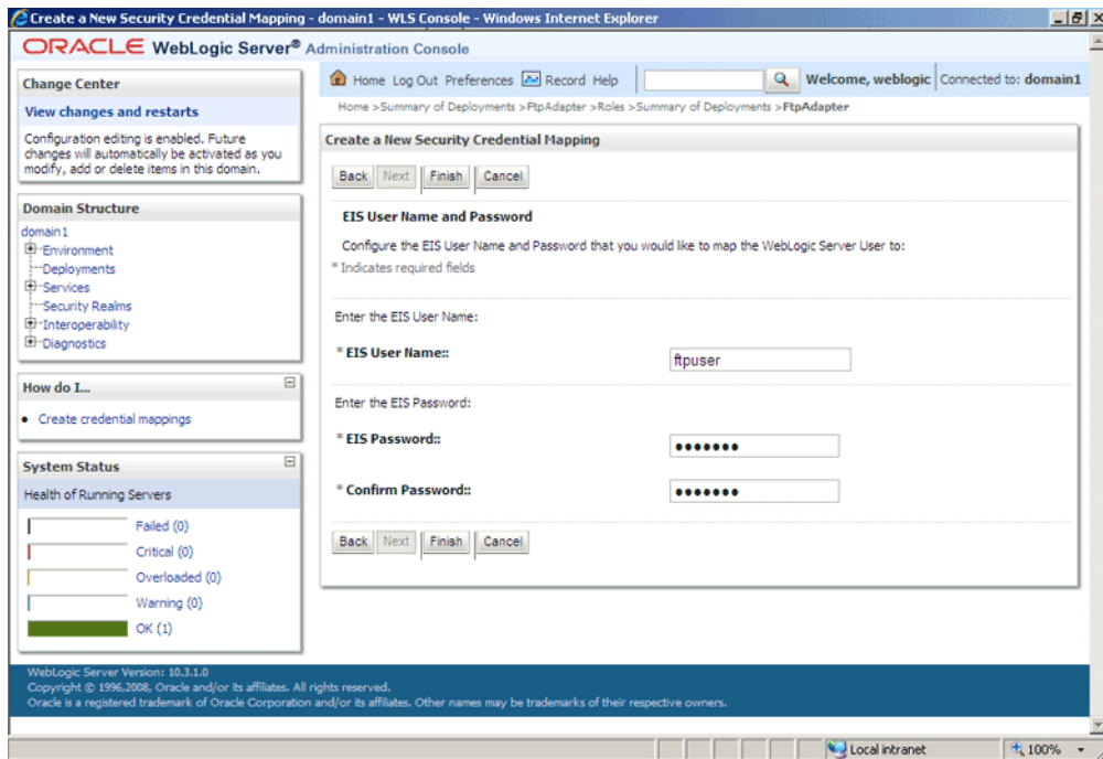
Figure 4–16 The Oracle WebLogic Server Administration Console - Create a New Security Credential Mapping Page
