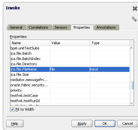
Figure 4–29 The Invoke Dialog
