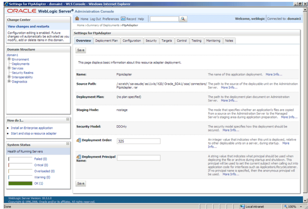
Figure 4-10 The Oracle WebLogic Server Administration Console - Settings for FTPAdapter Page
