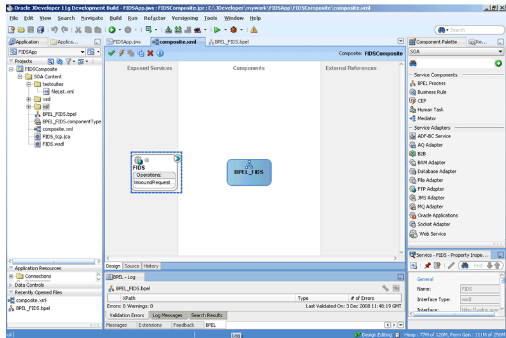
Figure 5–74 The JDeveloper - composite.xml Page
