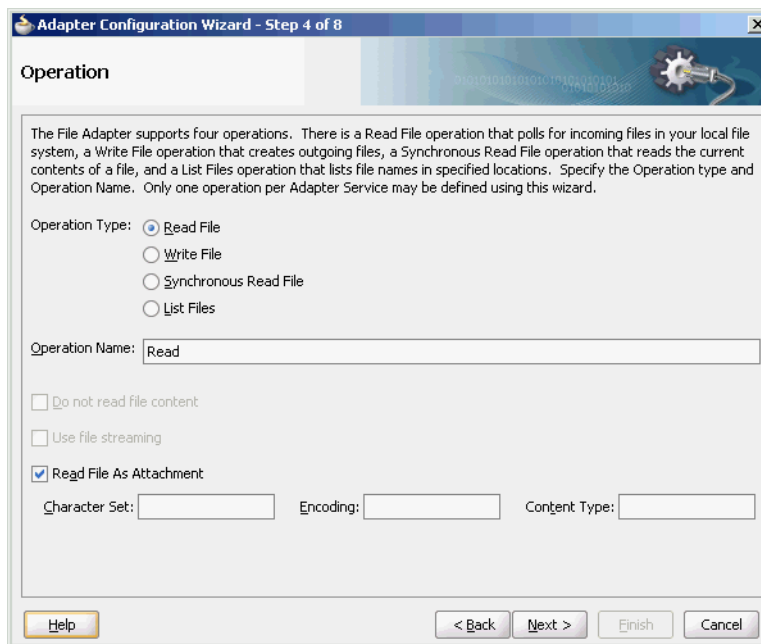
Figure 4–115 The Adapter Configuration Wizard Operation Page
