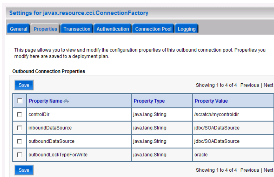
Figure 4-43 Oracle WebLogic Server Administration Console - Settings for javax.resource.cci.Connectionfactory Page
