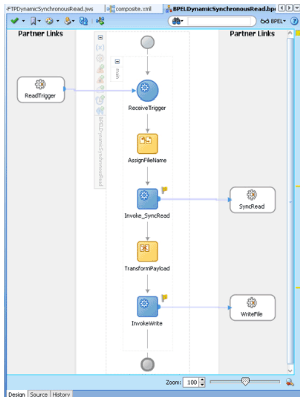
Figure 4–162 The JDeveloper - BPELDynamicSynchronousRead.bpel
