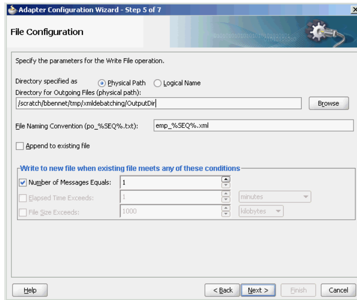
Figure 4–59 The Adapter Configuration Wizard - File Configuration Page
