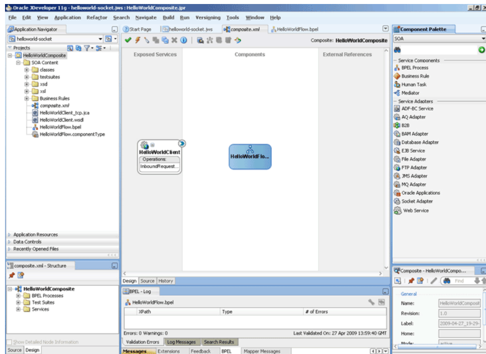
Figure 5-47 The JDeveloper - composite.xml Page
