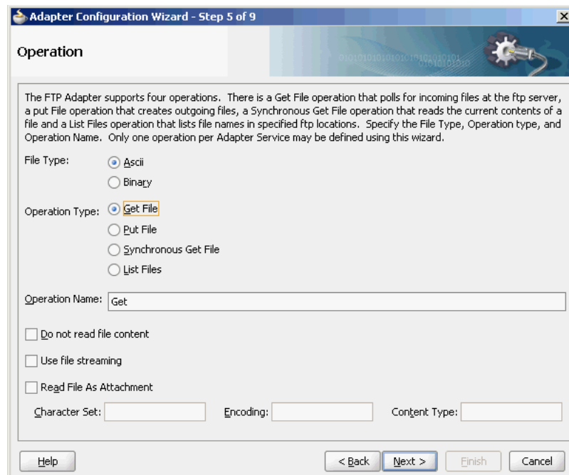
Figure 4–146 The Adapter Configuration Wizard Operation Page
