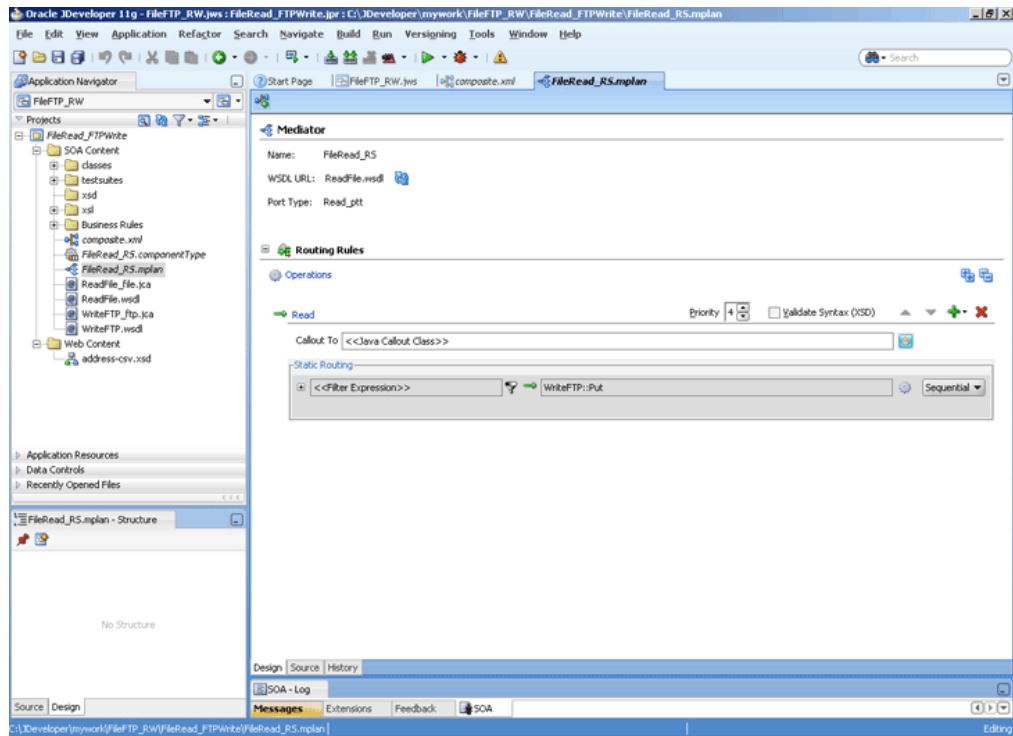
Figure 4–84 The JDeveloper - ReadFile_RS Routing Service Page
