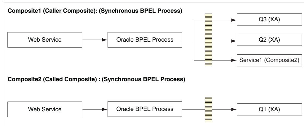
Figure 2–11 Sample Scenario: Handling Message Errors
