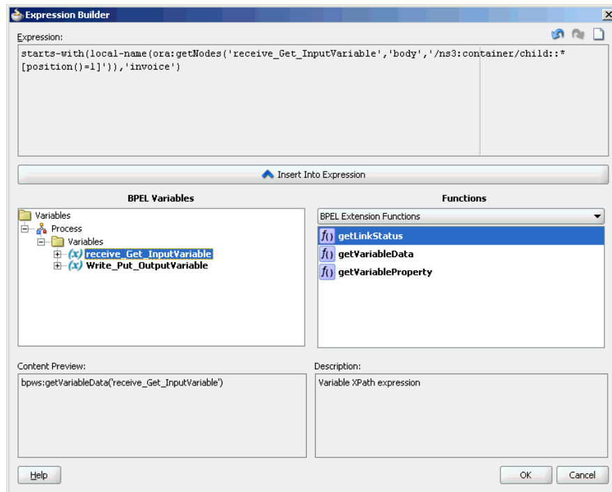
Figure 4–151 The Expression Builder Dialog
