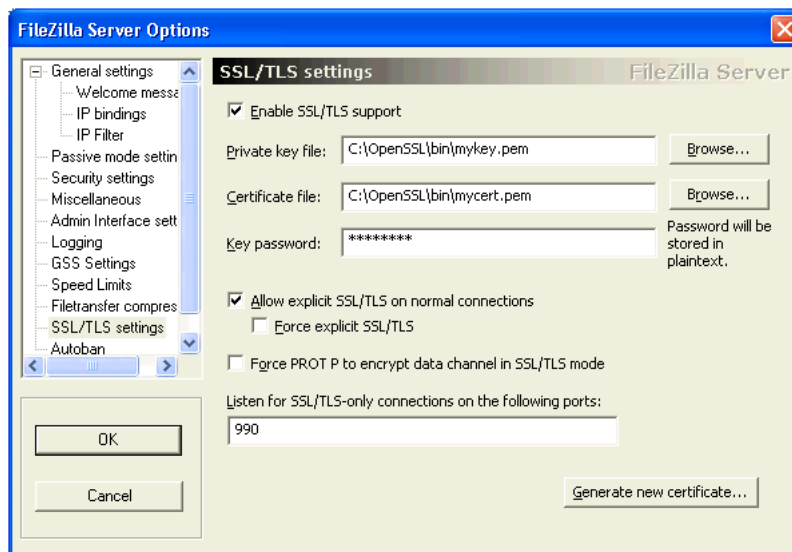
Figure 4-45 The FileZilla Server Options Dialog
