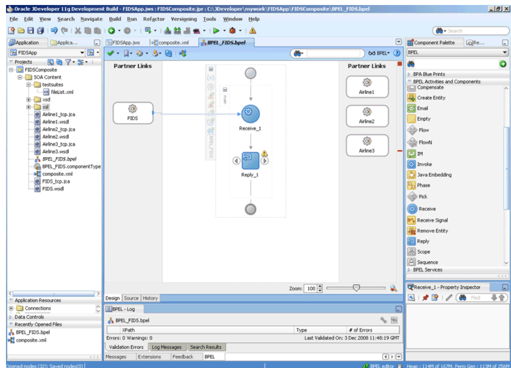
Figure 5–85 The JDeveloper - BPEL_FIDS.bpel
