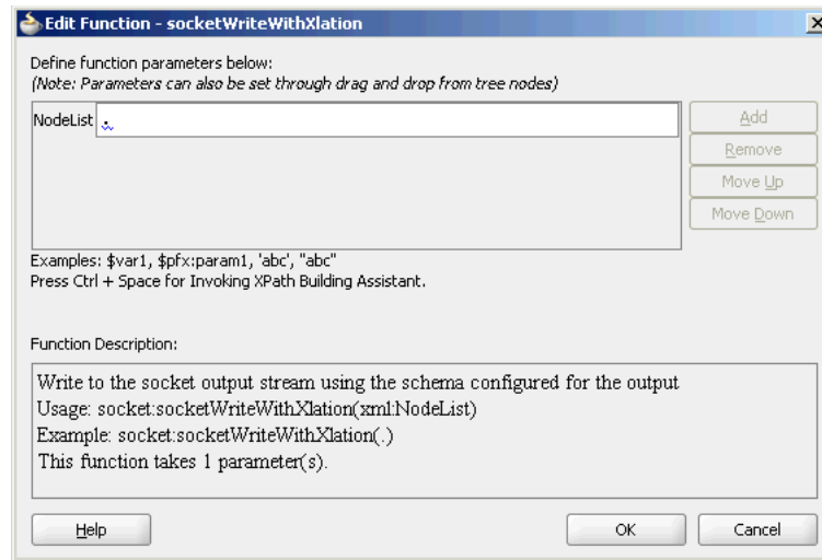
Figure 5–29 The Edit Function - socketWriteWithXlation Dialog
