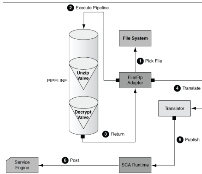
Figure 4–3 A Sample Pre-Processing Pipeline
