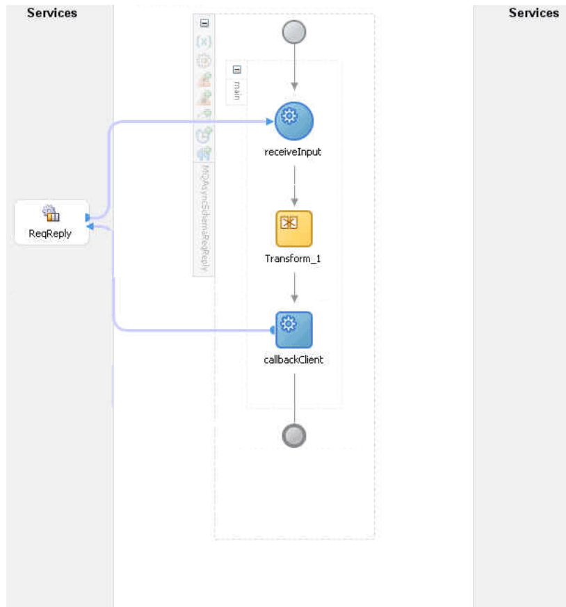
Figure 10–20 Asynchronous Request-Response Oracle BPEL PM As Server Sample
