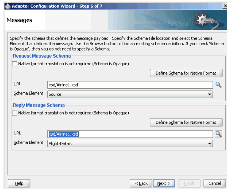
Figure 5–76 The Adapter Configuration Wizard - Messages Page
