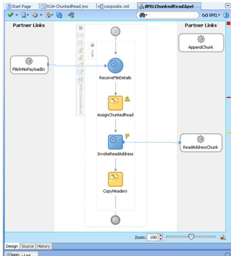
Figure 4–110 The JDeveloper - BPELChunkedRead.bpel
