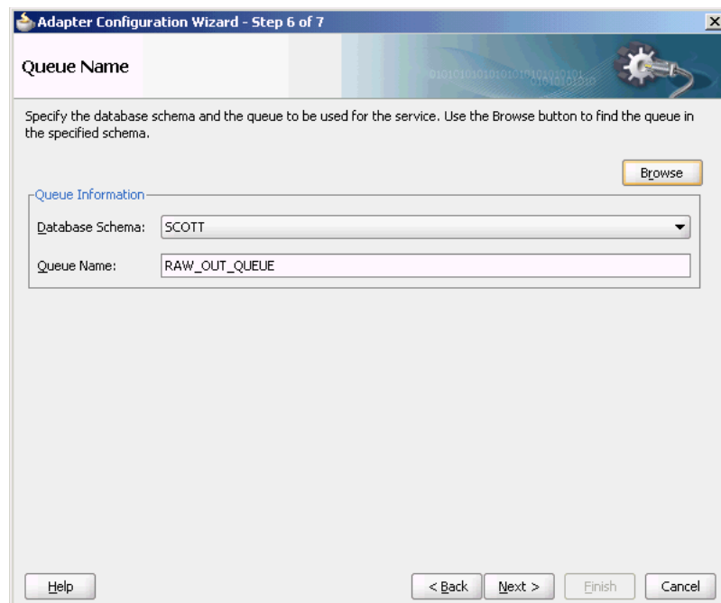
Figure 7-42 The Adapter Configuration Wizard Queue Name Page
