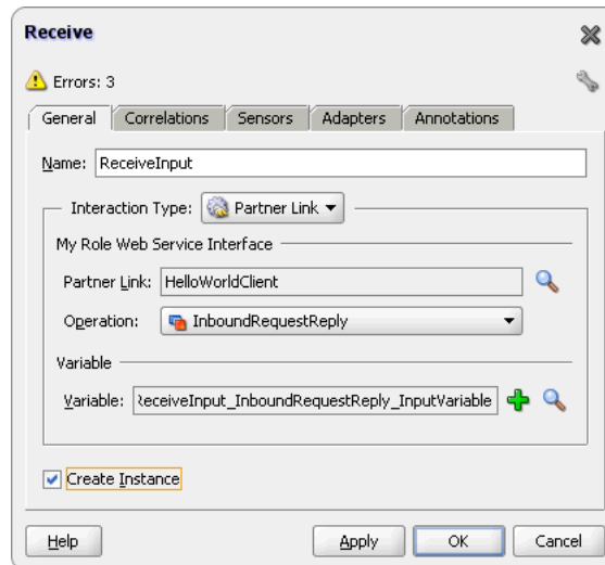
Figure 5–56 The Receive Dialog
