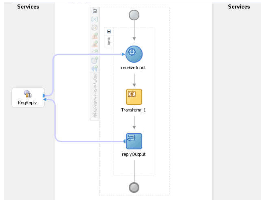
Figure 10–16 Synchronous Request-Response Oracle BPEL PM As Server Sample
