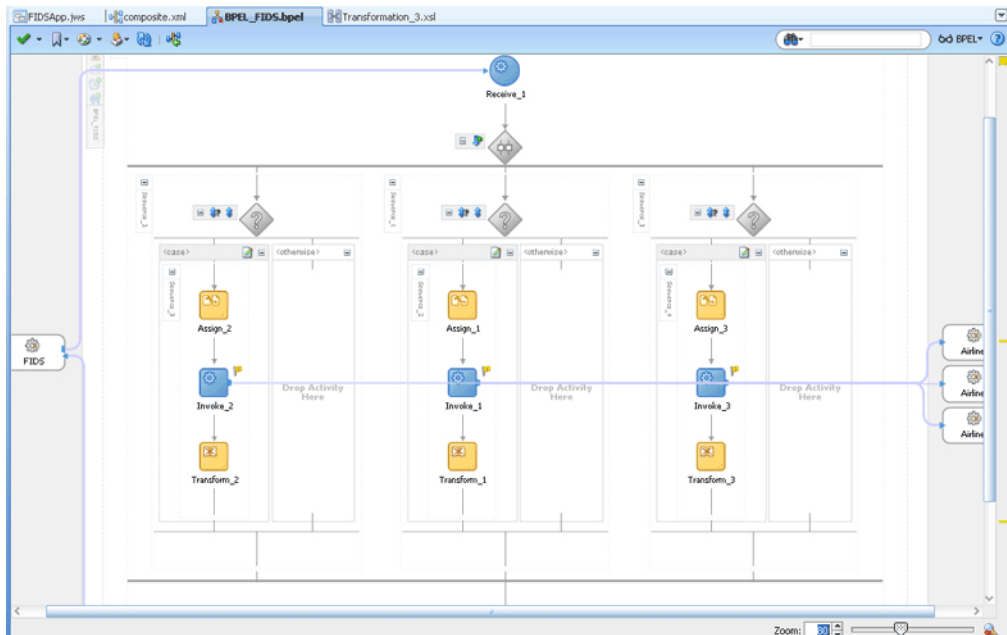
Figure 5–106 The JDeveloper - BPEL_FIDS.bpel
