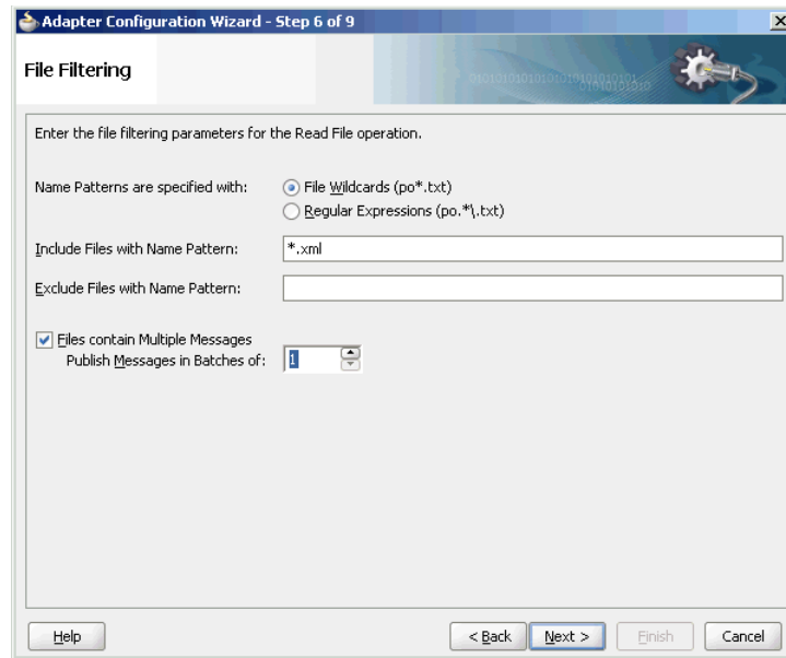
Figure 4–55 The Adapter Configuration Wizard File Filtering Page
