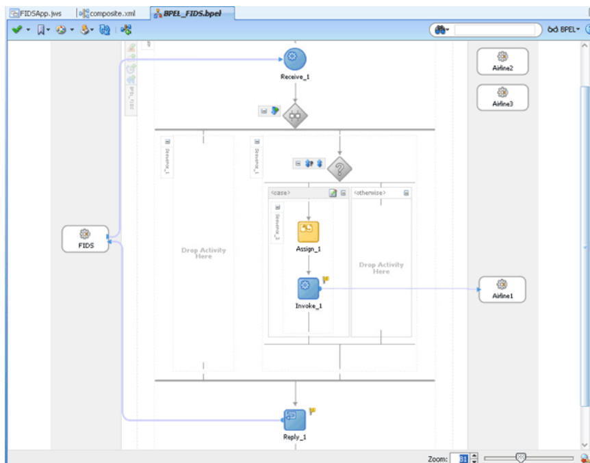
Figure 5–94 The JDeveloper - BPELFIDS.bpel
