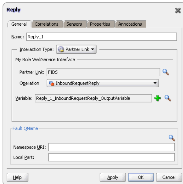
Figure 5-86 The Reply Dialog
