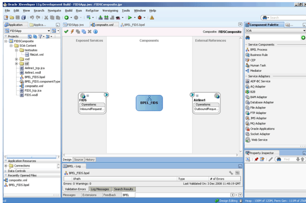
Figure 5–78 The JDeveloper - composite.xml Page
