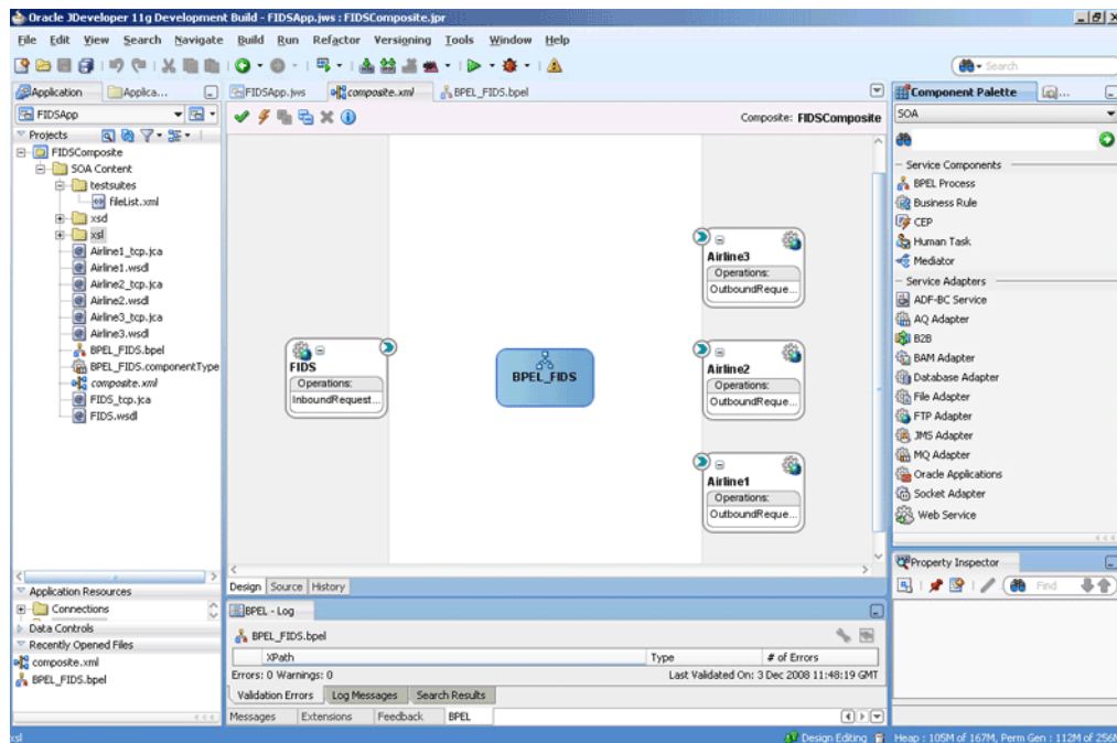
Figure 5–80 The JDeveloper - composite.xml Page
