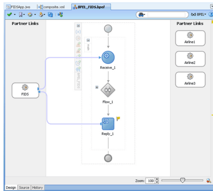
Figure 5–88 The JDeveloper - BPEL_FIDS.bpel
