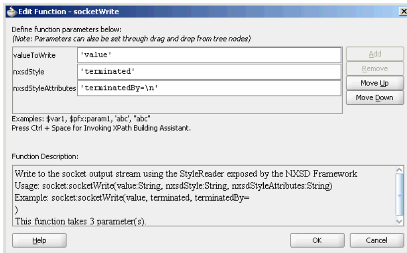
Figure 5–22 The Edit Function - socketWrite Dialog
