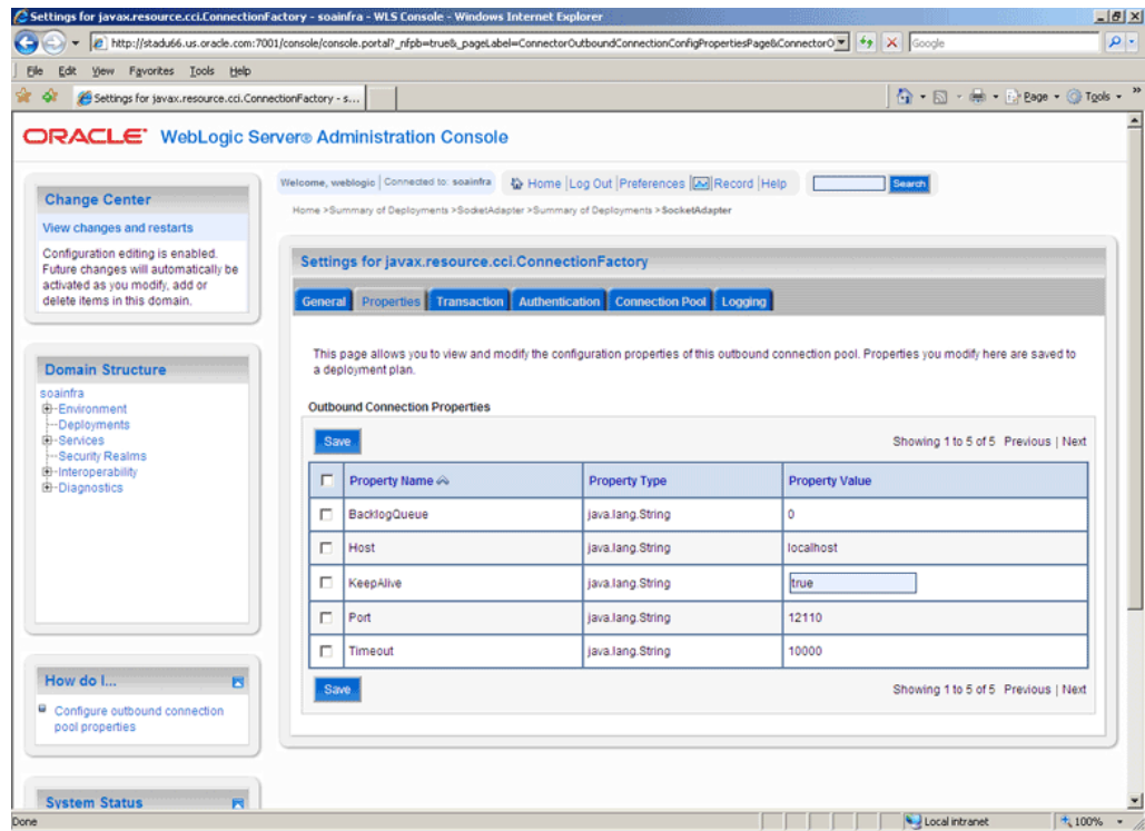
Figure 5–13 Oracle WebLogic Server Console - Settings for javax.resource.cci.ConnectionFactory Page
