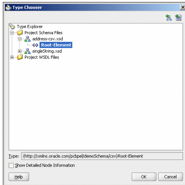
Figure 4–86 The Type Chooser Dialog
