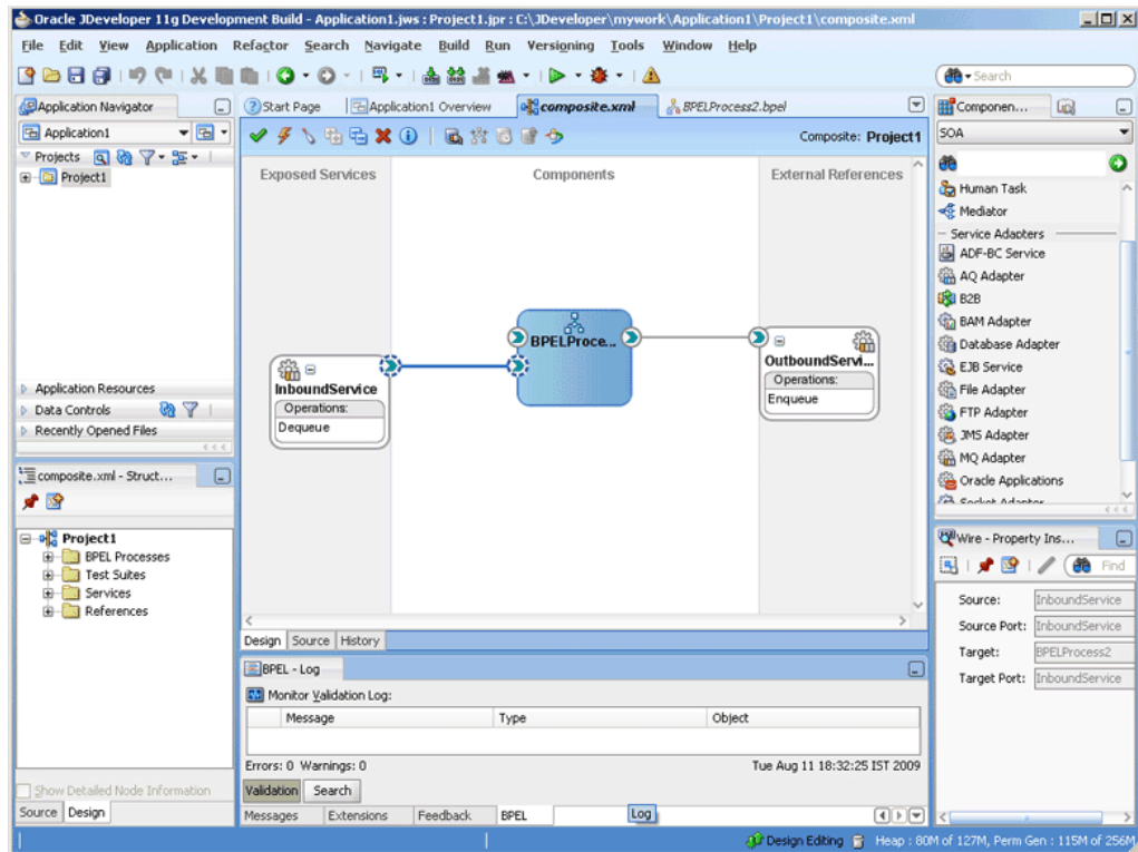
Figure 10–92 The JDeveloper - Composite.xml
