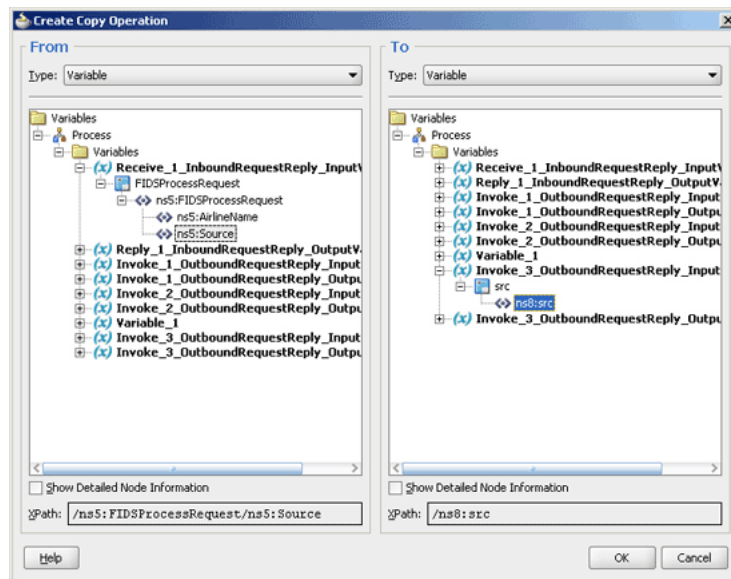
Figure 5–103 The Create Copy Operation Dialog
