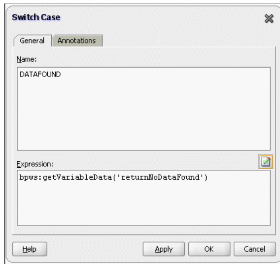
Figure 4–111 The Switch Case Dialog
