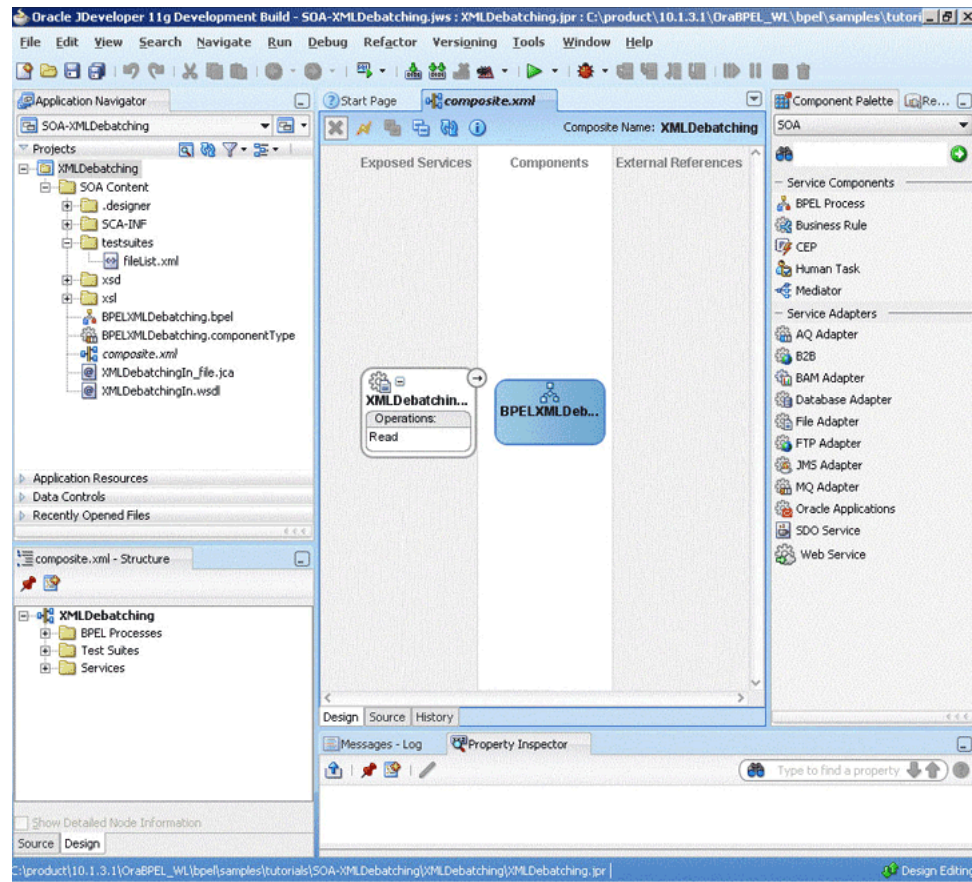
Figure 4–58 The JDeveloper - Composite.xml
