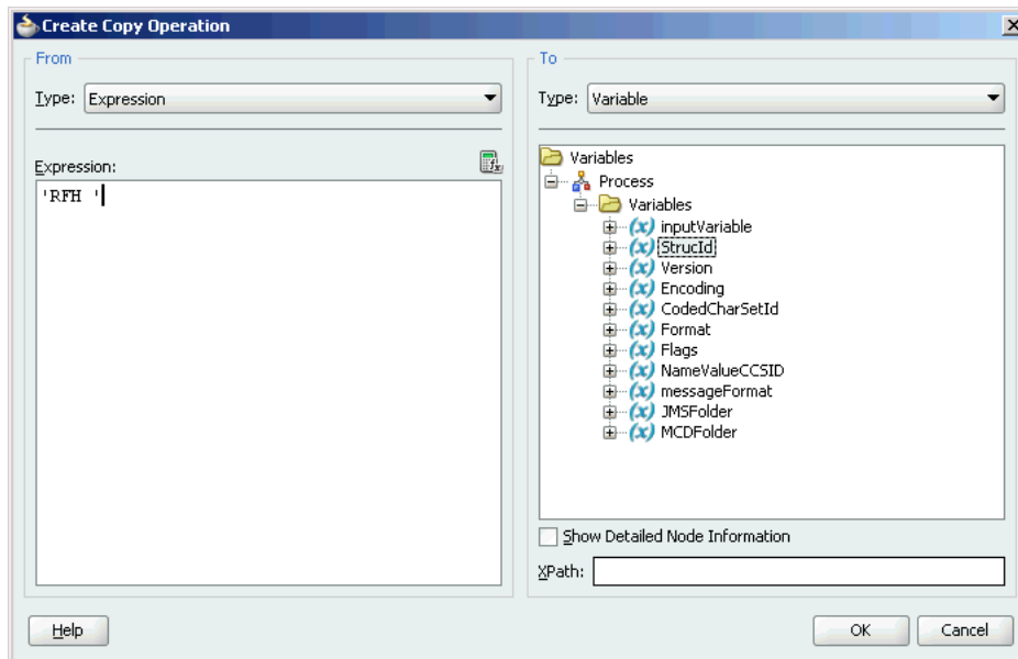
Figure 10–95 The Create Copy Operation Dialog
