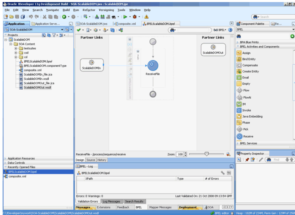
Figure 4–91 The JDeveloper - BPELScalableDOM.bpel
