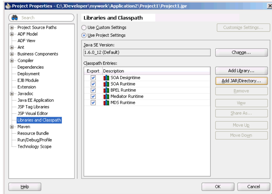
Figure 4-4 The Project Properties Dialog
