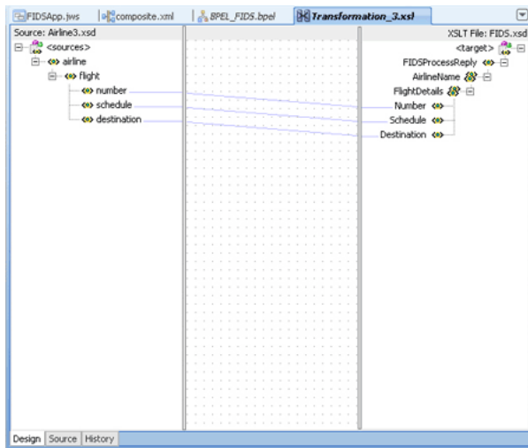
Figure 5–105 The Transformation_3.XSL Page
