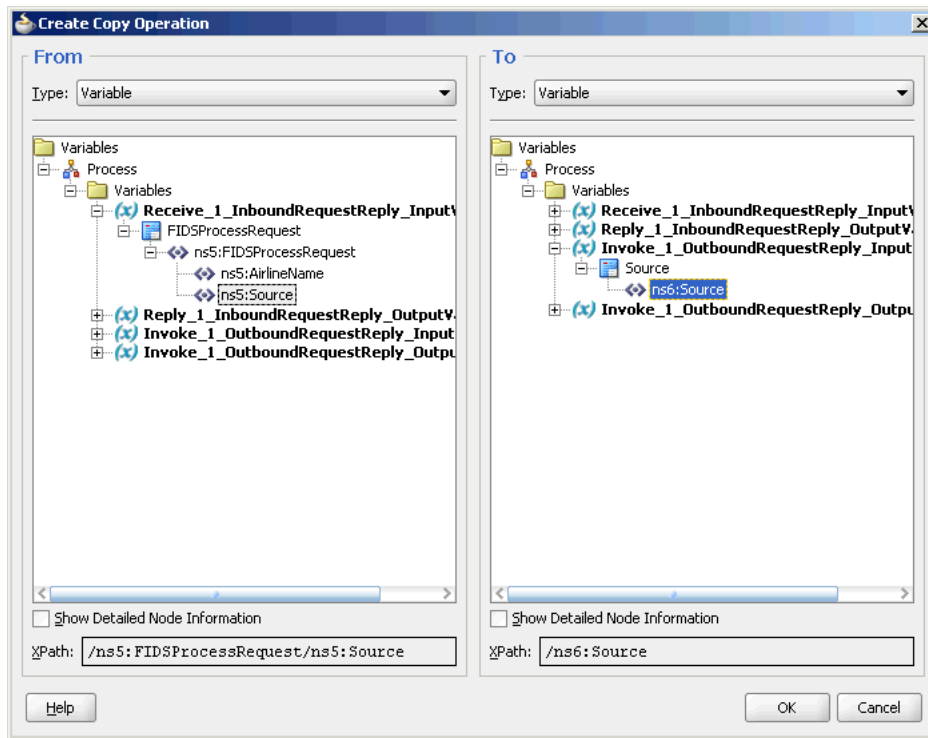
Figure 5–93 The Create Copy Operation Dialog
