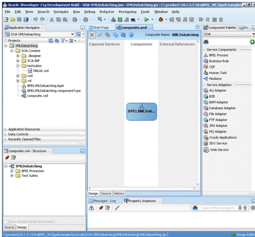
Figure 4–51 The JDeveloper - Composite.xml
