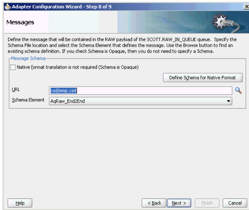
Figure 7–40 The Adapter Configuration Wizard Messages Page
