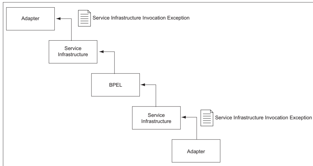
Figure 2–10 Fault Propagation
