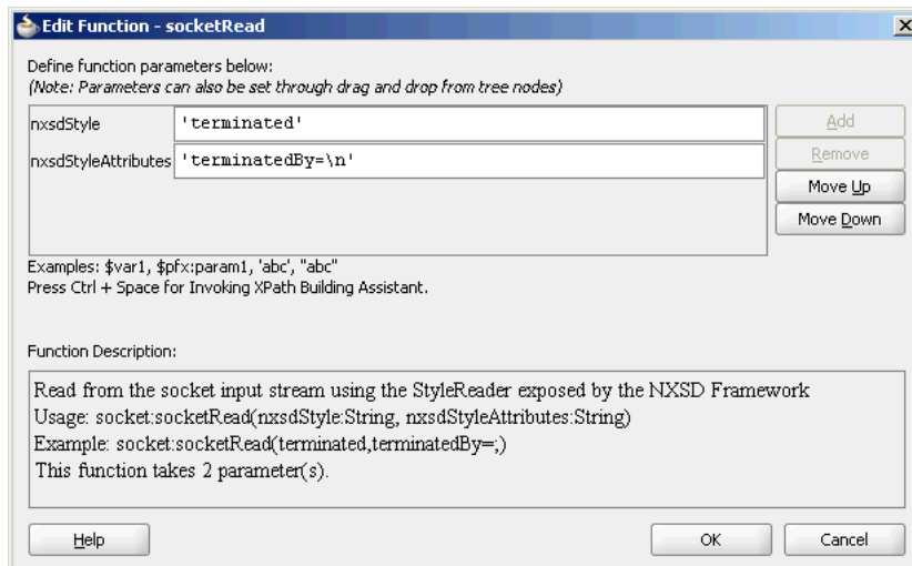
Figure 5–20 The Edit Function - socketRead Dialog
