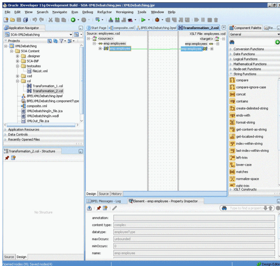
Figure 4–74 The JDeveloper - Transformation_2.xsl
