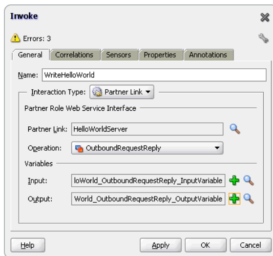
Figure 5–61 The Invoke Dialog
