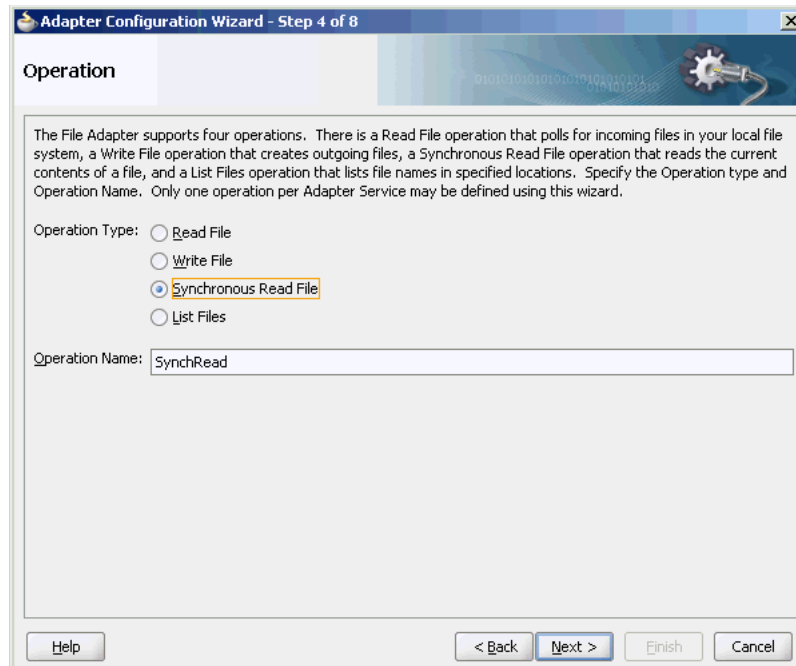
Figure 4–31 Synchronous Read Operation Page
