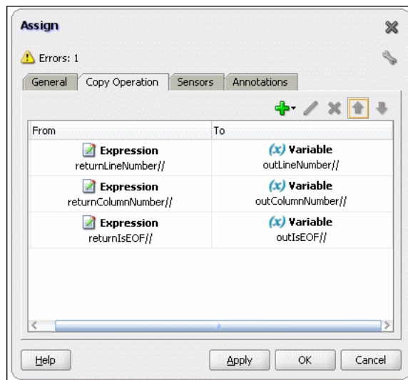
Figure 4-109 The Assign Dialog
