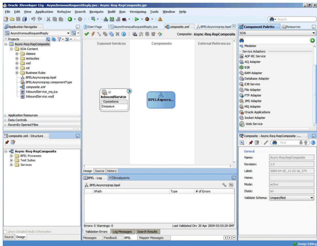
Figure 10-73 The JDeveloper Page - Composite.xml Page
