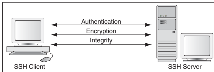
Figure 4–46 SFTP Communication
