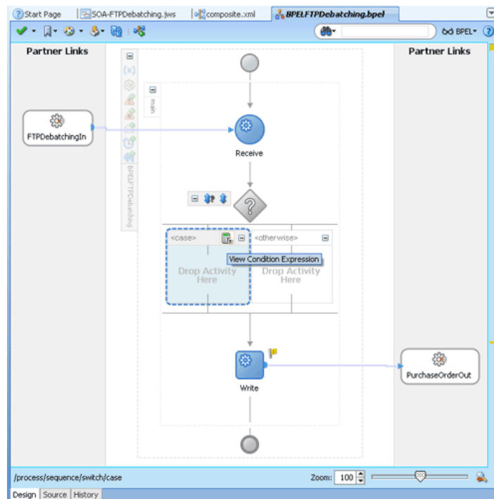
Figure 4-150 BPELFTPDebatching.bpel Page
