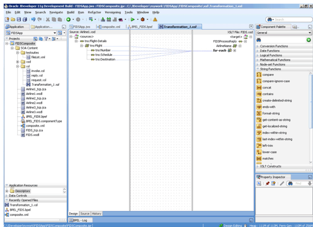
Figure 5–95 The JDeveloper - Transformation_1.XSL Page
