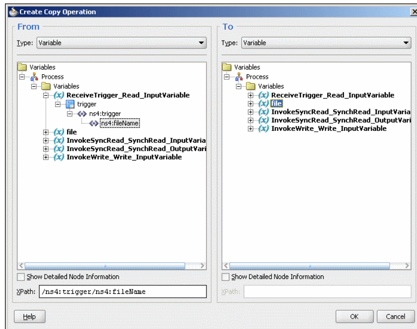
Figure 4–160 The Create Copy Operation Dialog
