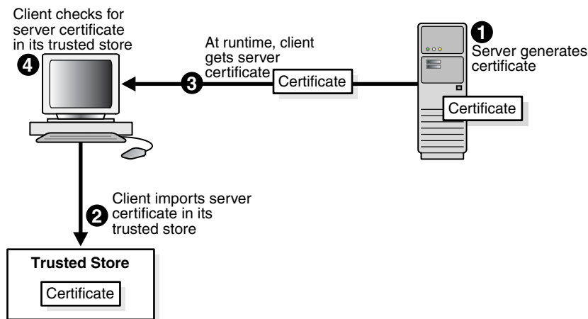
Figure 4-44 Establishing Trust
