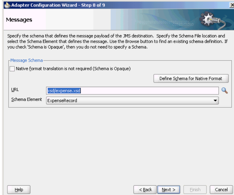
Figure 8–12 Completed Messages Dialog
