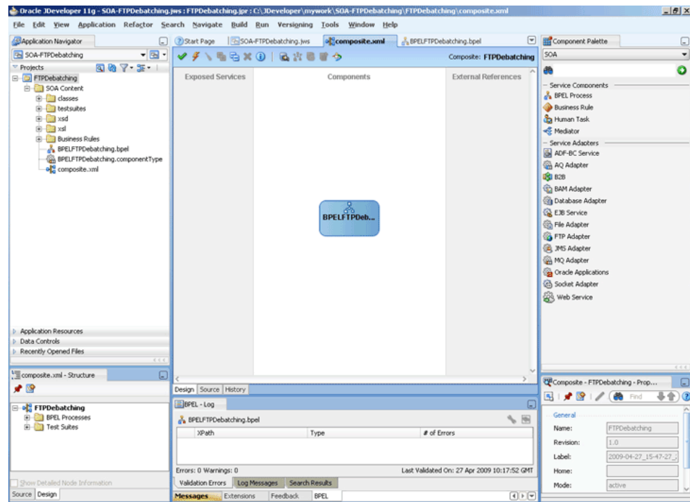
Figure 4-144 The JDeveloper - Composite.xml
