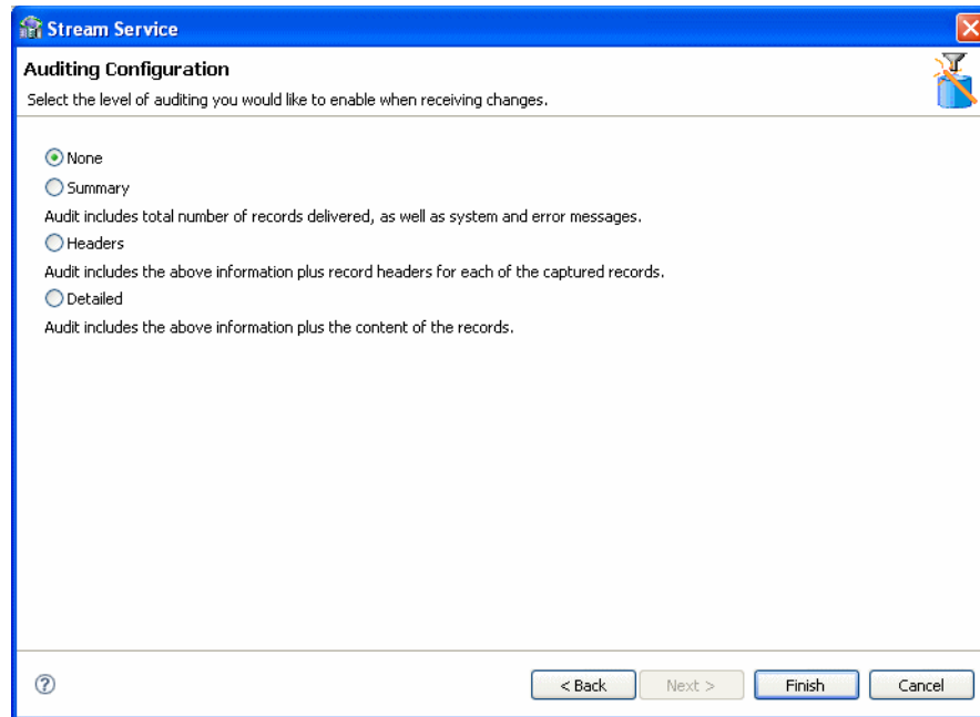
Figure 2–37 Auditing Configuration
