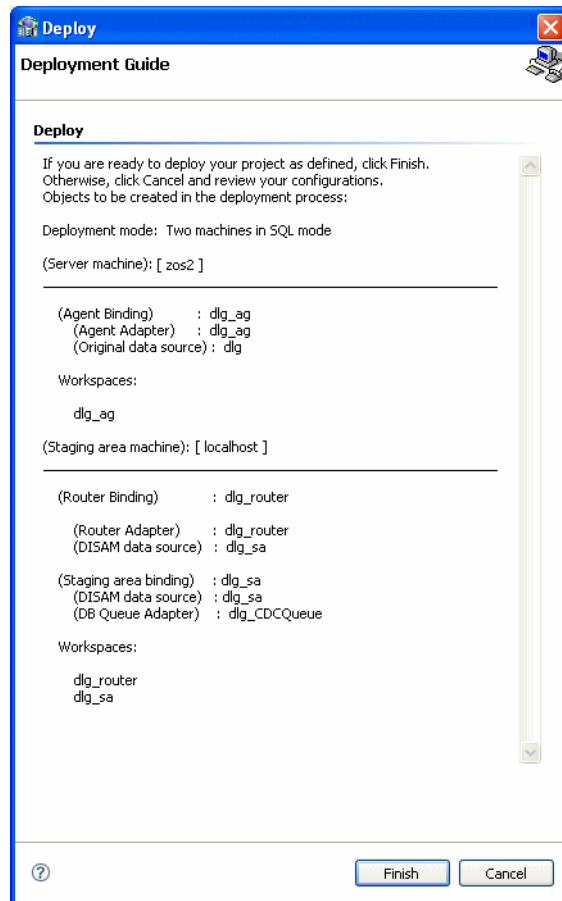
Figure 2–42 Deployment Guide
