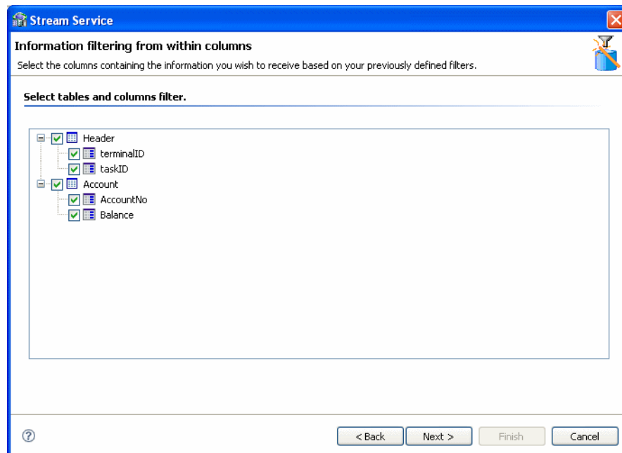
Figure 2–32 Column Selection
