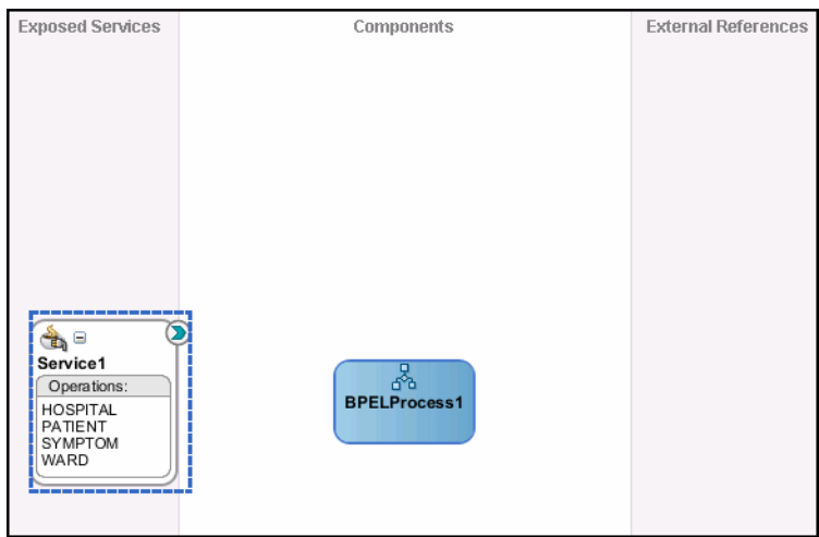
Figure 5-3 BPEL Process
