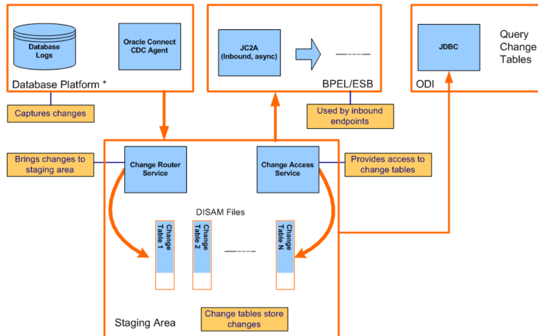
Figure 1-1 Component Architecture used with the VSAM CDC adapter
