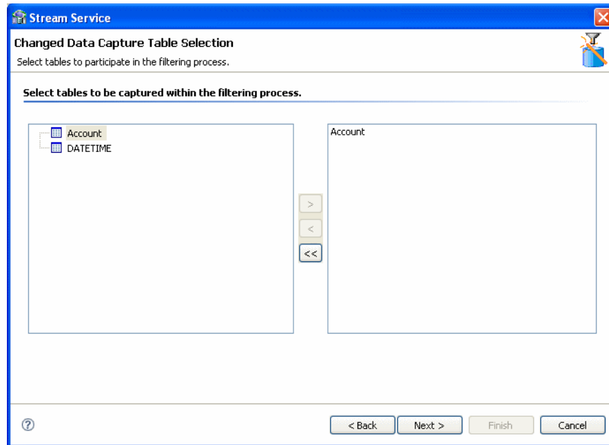
Figure 2–31 Select Tables
