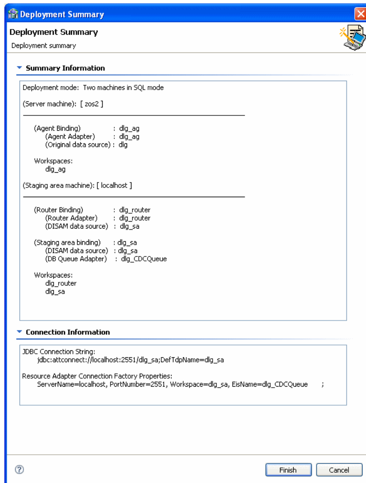
Figure 2–43 Deployment Summary
