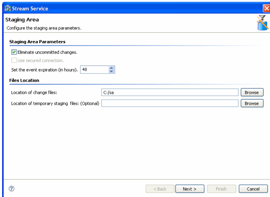
Figure 2–30 Staging Area
