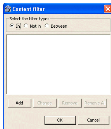
Figure 2–34 Content Filter
