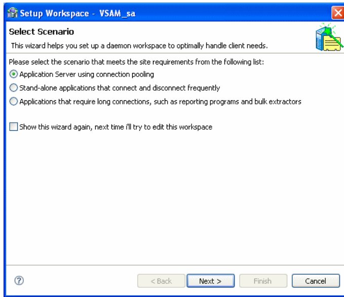
Figure 2–38 Select Scenario
