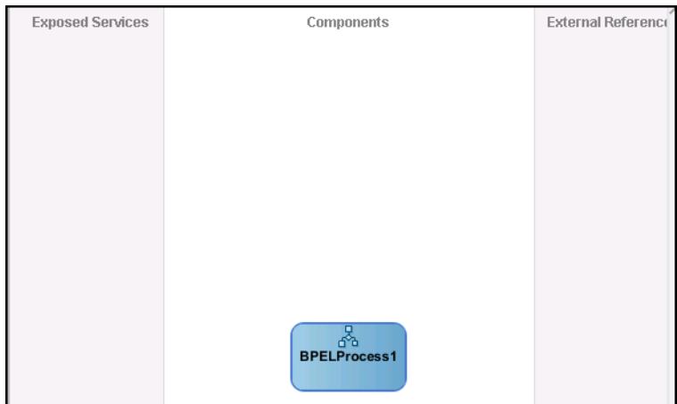
Figure 5-4 Composite View
