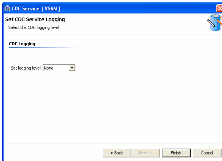
Figure 2–29 Logging Level
