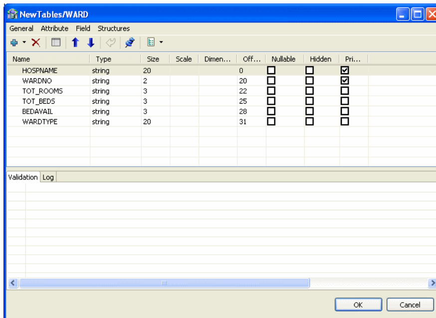
Figure 2–27 Field Manipulation
