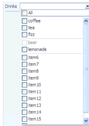
Figure 9–24 selectManyChoice Component
