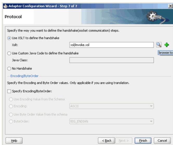
Figure 5–8 Defining a Protocol with Handshake Mechanism By Using a Style Sheet
