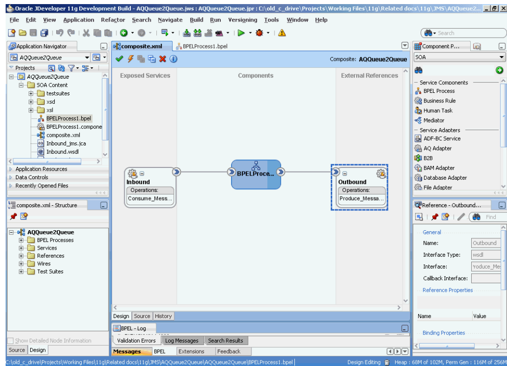
Figure 8–25 JDeveloper - Composite.xml
