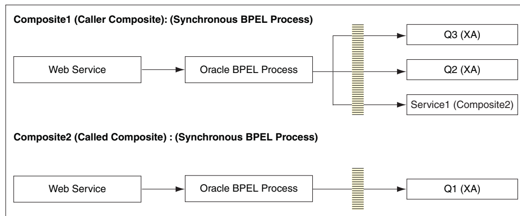
Figure 2–13 Sample Scenario: Handling Message Errors
