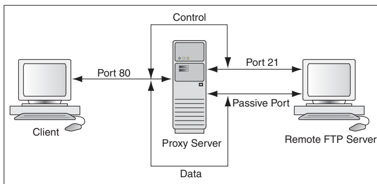
Figure 4–3 Remote FTP Server Communication Through a Proxy Server
