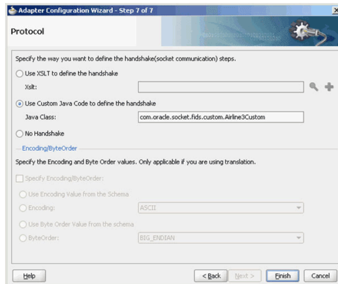
Figure 5–9 Defining a Protocol with Handshake Mechanism By Using Custom Java Code
