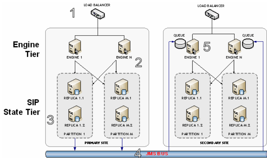
Figure 4–2 Geo-Redundancy
