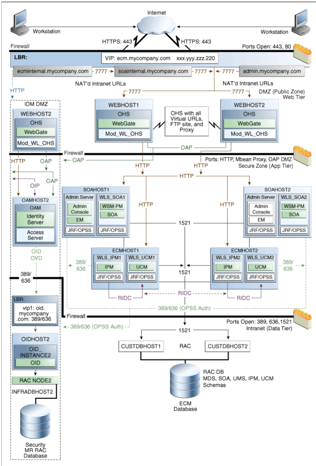
Figure 4-10 Reference Topology for Oracle ECM Enterprise Deployment
