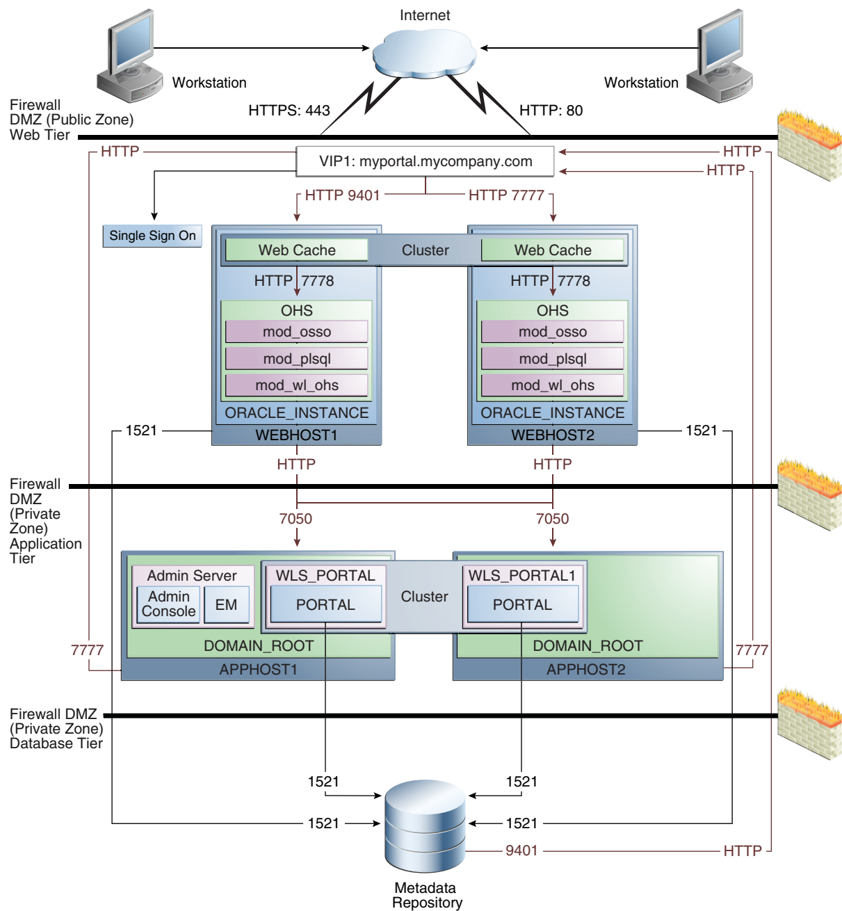
Figure 4–7 Oracle Portal Topology Diagram
