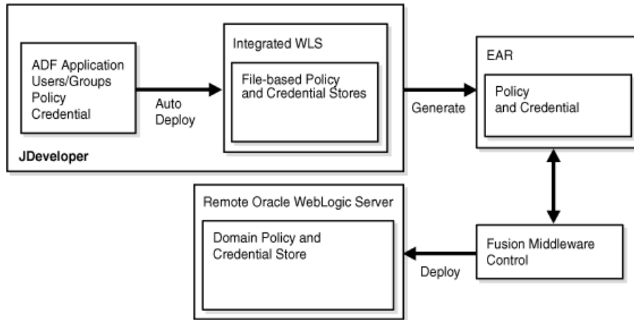
Figure 13–9 Oracle ADF Application Deployed to Oracle WebLogic Server
