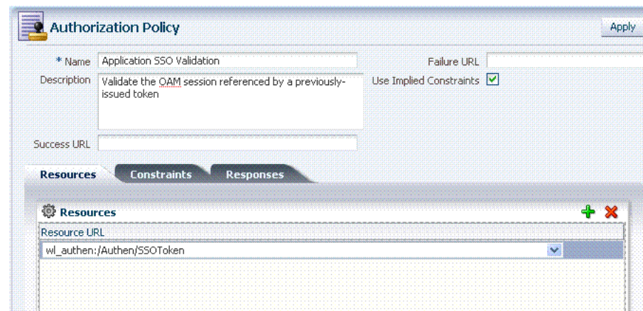
Figure 9–8 Pre-seeded Application SSO Authorization Policy and Resources
