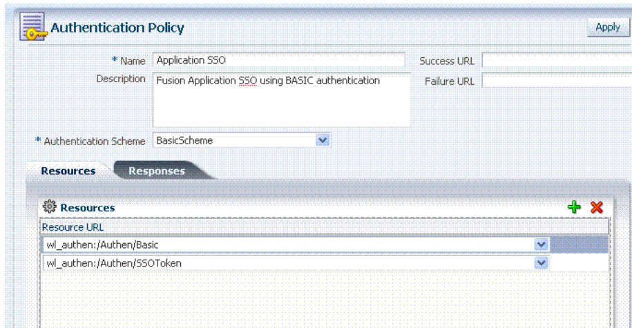
Figure 9–6 Pre-seeded Application SSO Authentication Policy and Resources
