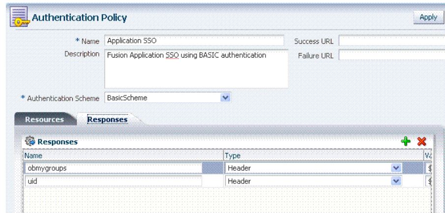
Figure 9–7 Pre-seeded Responses for the Application SSO Authentication Policy
