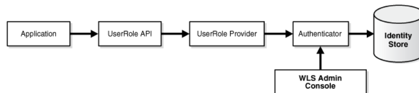
Figure 13–6 Searching the Identity Store with User and Role API
