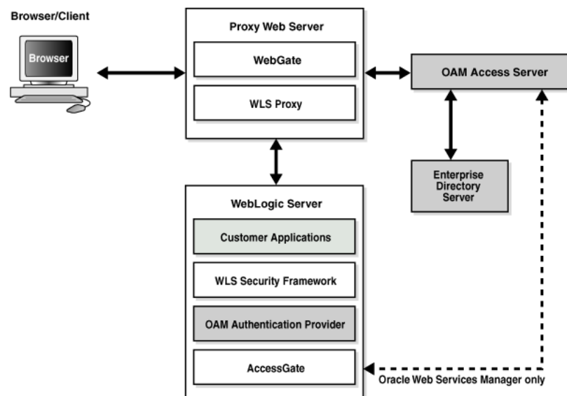
Figure 9–2 Identity Asserter Single Sign-On Solution for Web Resources Only
