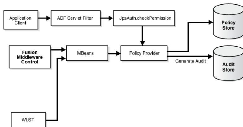
Figure 13–8 Oracle ADF using JpsAuth.checkPermission
