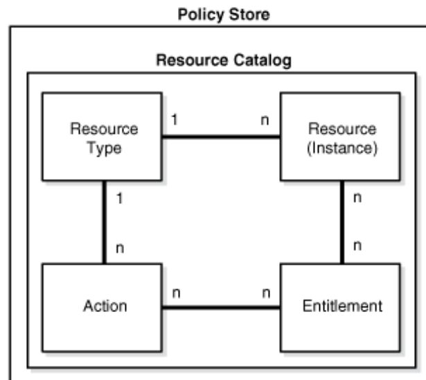
Figure 17-1 The Resource Catalog Logical Model
