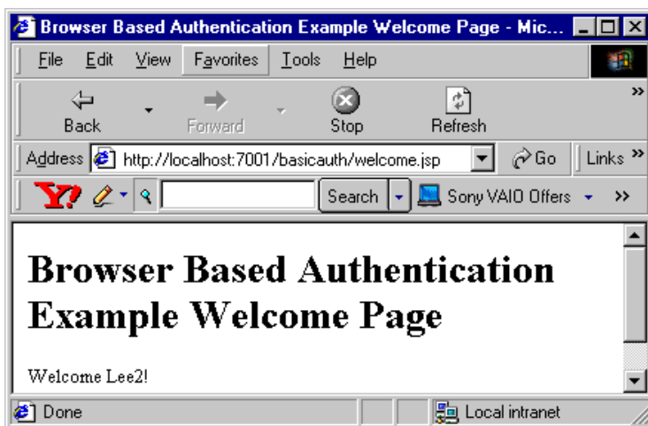
Figure 3-3 Welcome Screen
