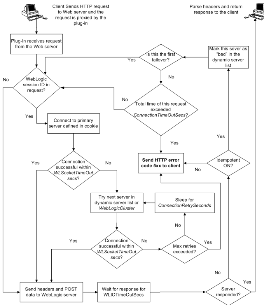
Figure 3-1 Connection Failover
