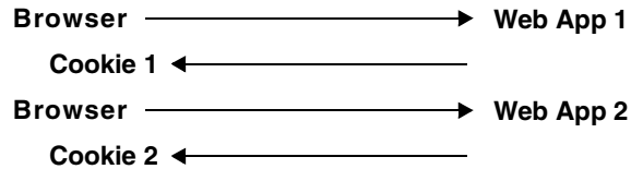
Figure 7-1 Cookies are Overwritten
