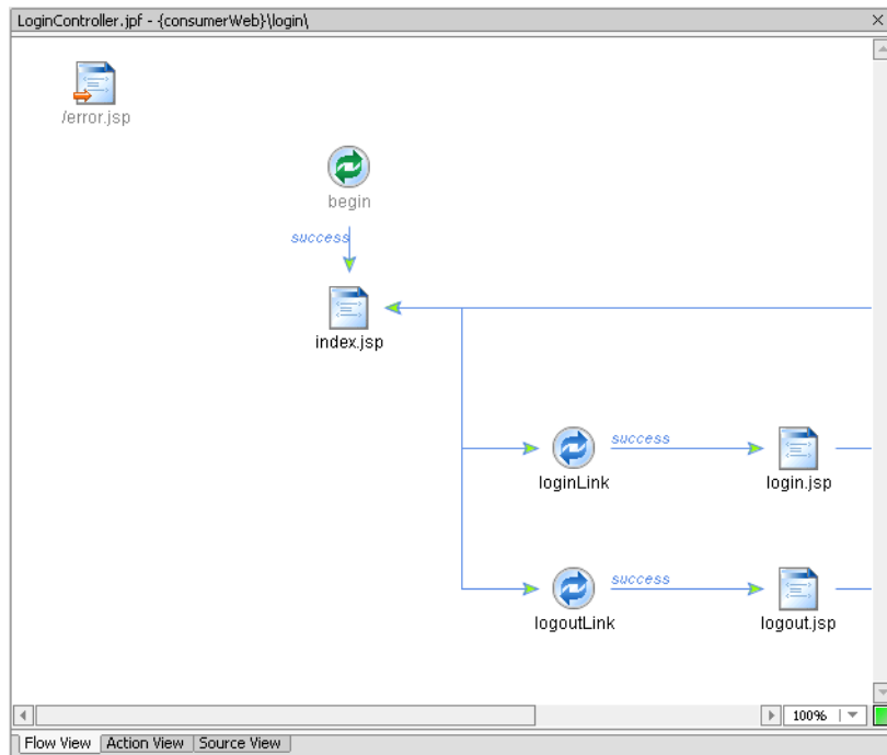
Figure 9-4 LoginController.jspf Page Flow in IDE Workspace
