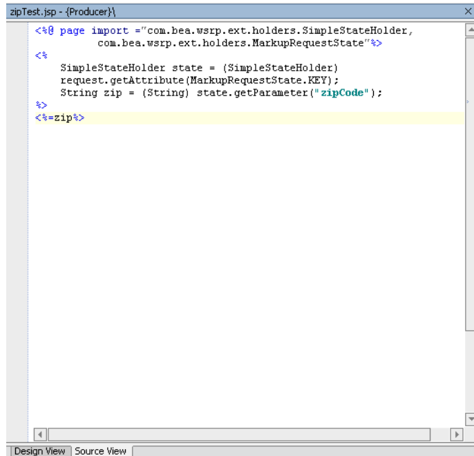
Figure 6-5 New JSP Source for zipTest.jsp
