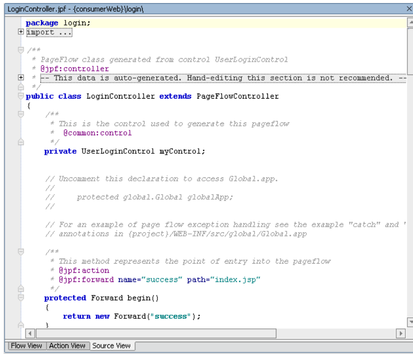
Figure 9-5 LoginController.jpf Source
