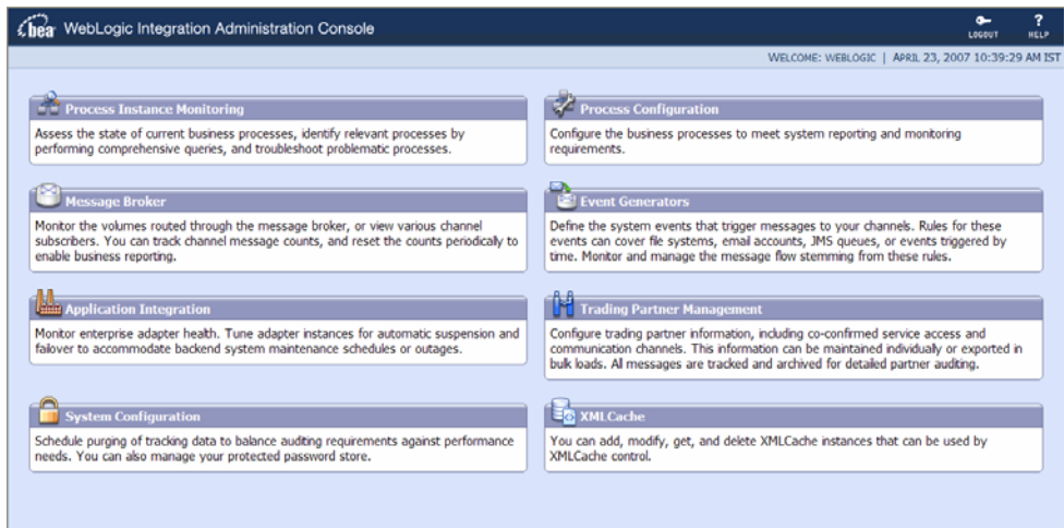
Figure 1-2 WebLogic Integration Administration Console
