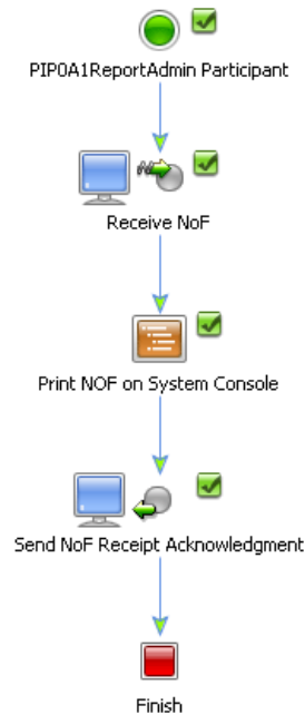
Figure 2-5 Report Administrator Business Process
