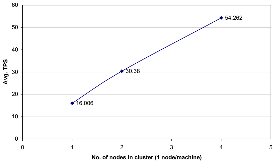
Figure A-5 Results of Horizontal Scalability Tests
