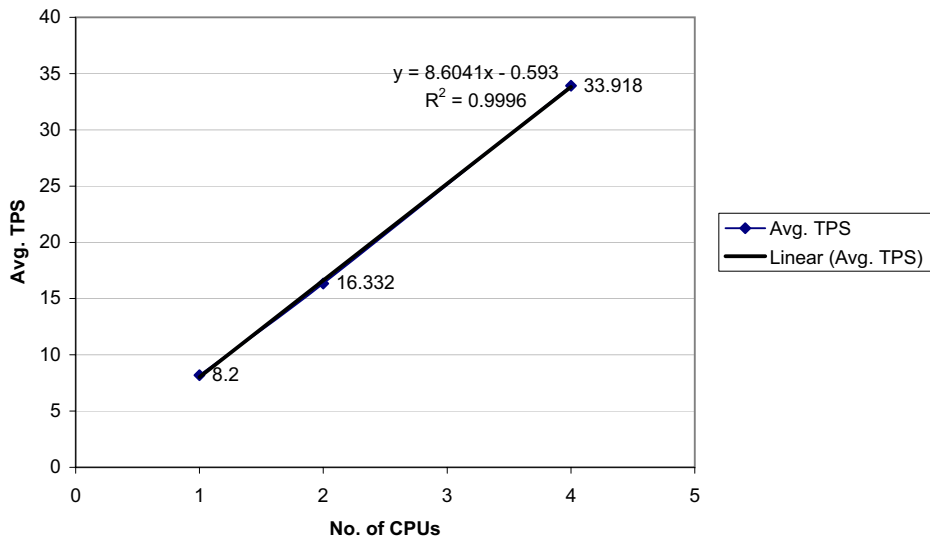
Figure A-6 Capacity Estimation: Vertical Scaling
