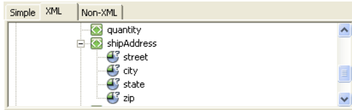
Figure 9-3 XML Schema
