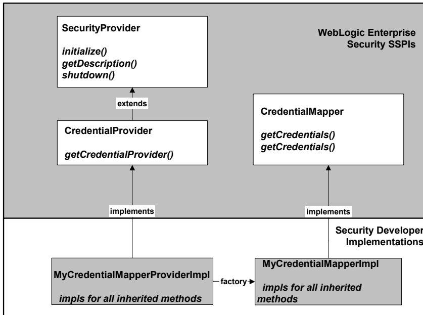
Figure 3-4 Credential Mapping SSPI and Two Runtime Classes
