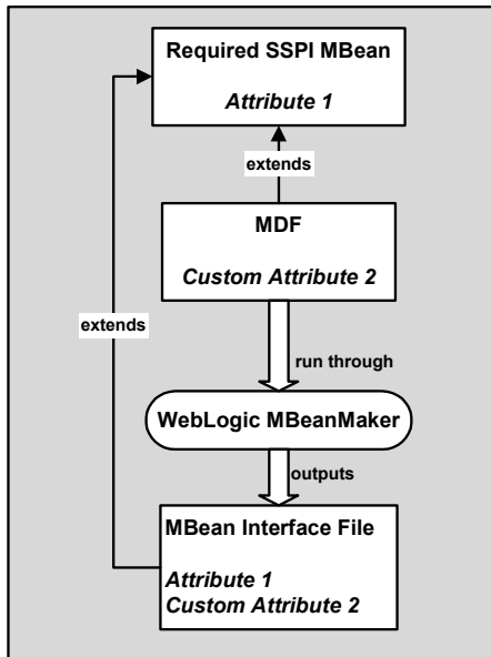
Figure 3-8 What the WebLogic MBeanMaker Provides
