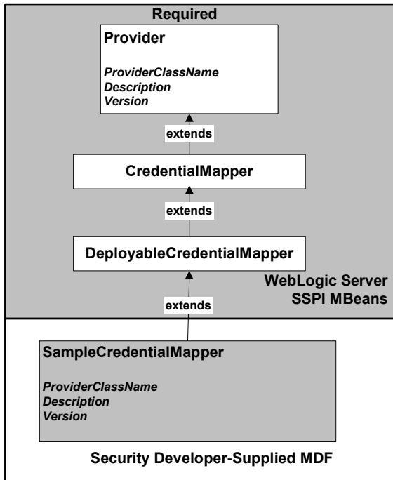
Figure 3-6 SSPI MBean Hierarchy for Credential Mapping Providers
