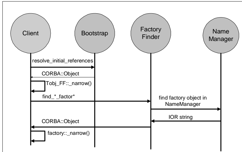
Figure 5-2 Locating a Factory Object
