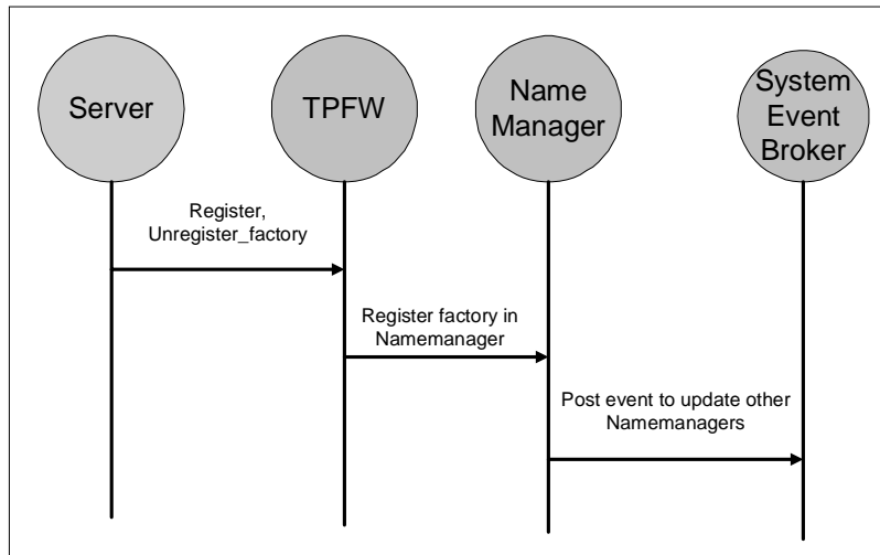
Figure 5-1 Registering a Factory Object
