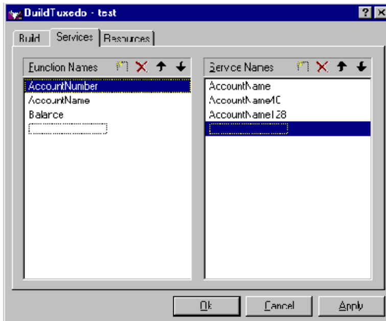
Figure 3-3 Services Page
