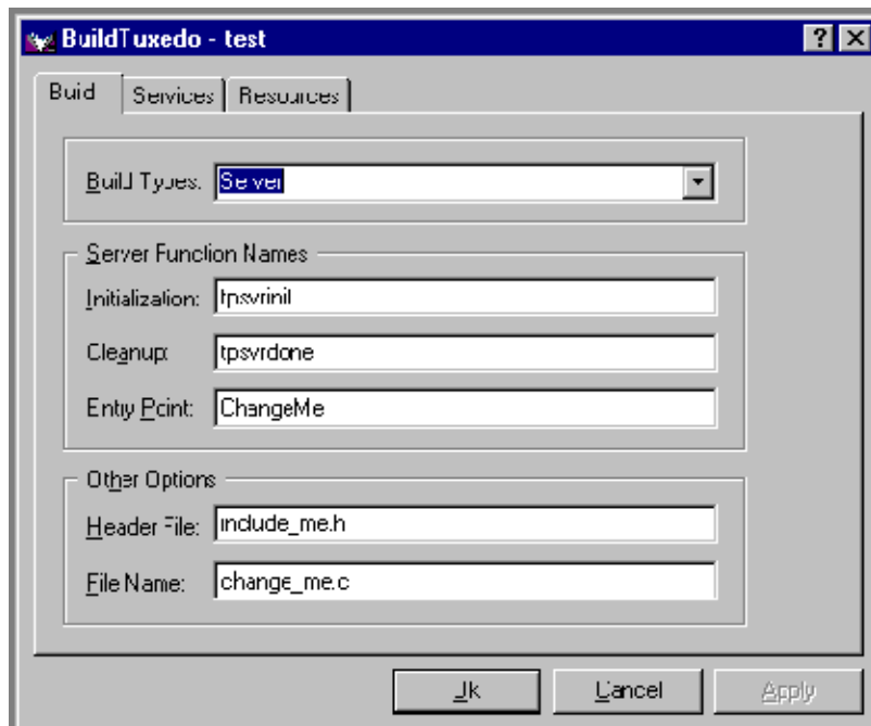
Figure 3-2 Build Page
