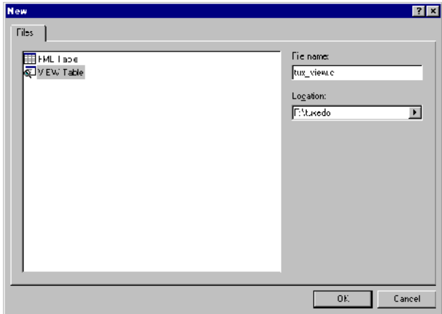
Figure 3-5 New Window
