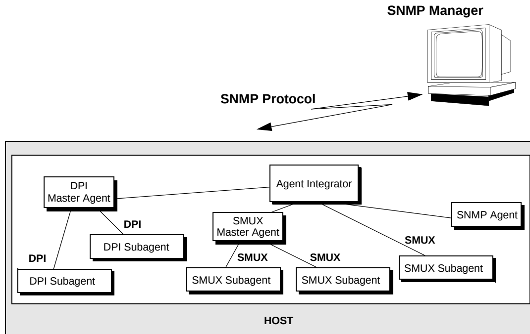
Figure 5-2 BEA SNMP Agent Integrator Master/Subagent Architecture
