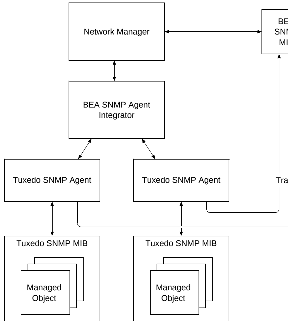
Figure 1-4 BEA SNMP Agent Components
