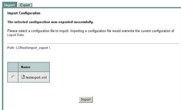
Figure 14-1 Import /Export Tab on the Liquid Data Node
