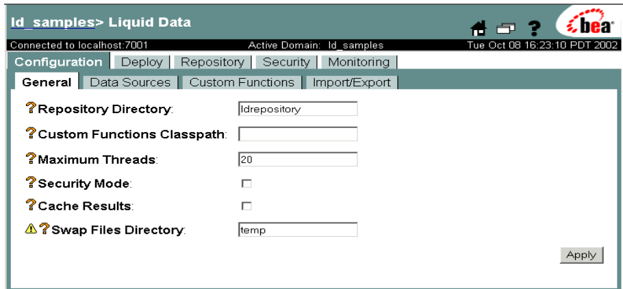
Figure 5-1 Configuring Liquid Data Server Settings
