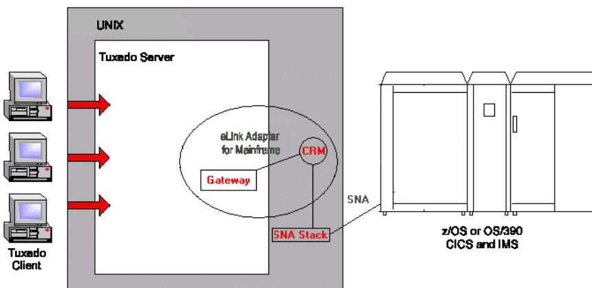
Figure 1-1 eLink Adapter for Mainframe Local Configuration
