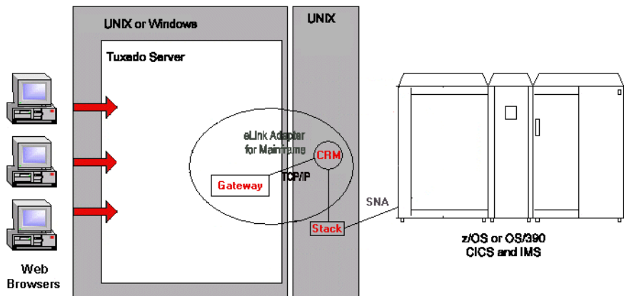
Figure 1-3 Non-Mainframe eLink Adapter for Mainframe Distributed Configuration
