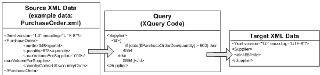
Figure 2-6 If-Then-Else
