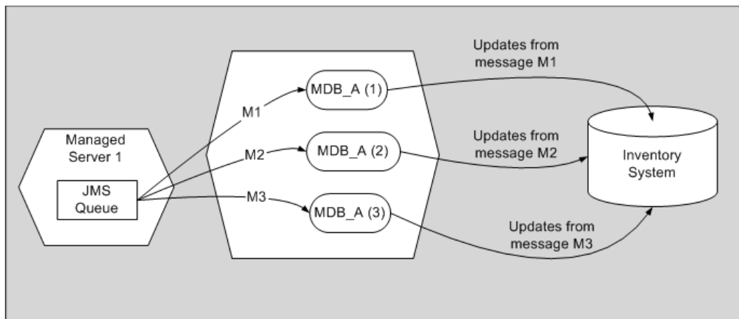
Figure 7-2 Point-to-Point Model
