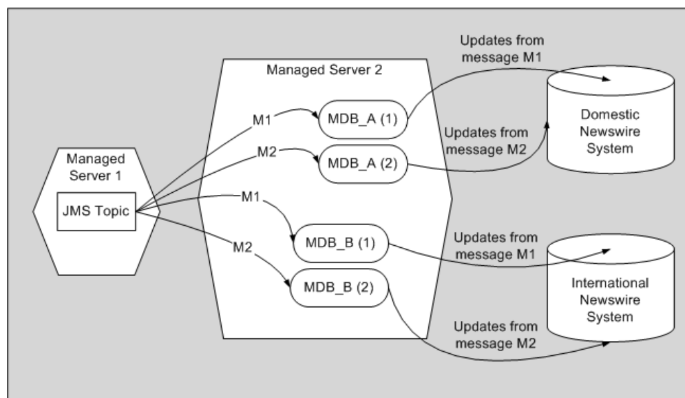
Figure 7-3 Publish/Subscribe Model
