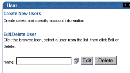
Figure 7–11 User Portlet
