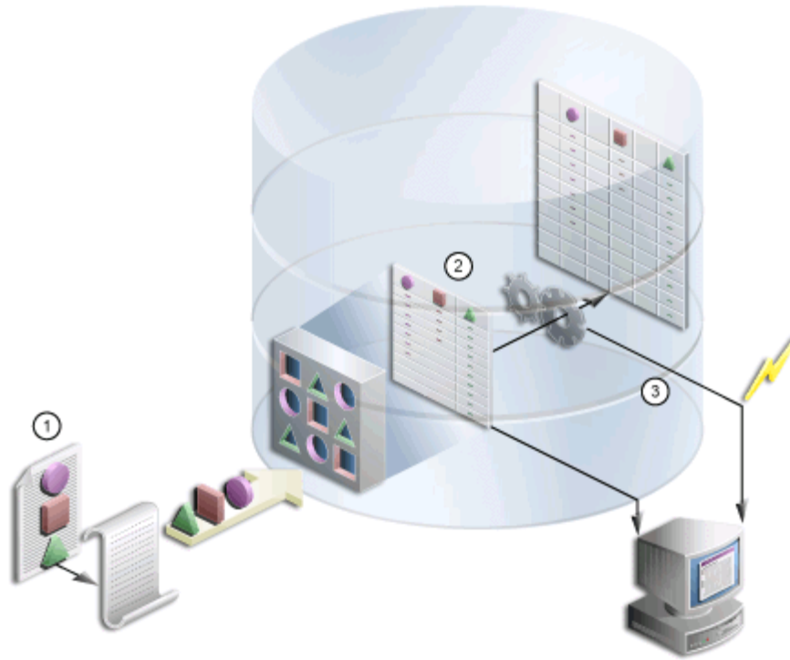
Figure 11–18 Import Process
