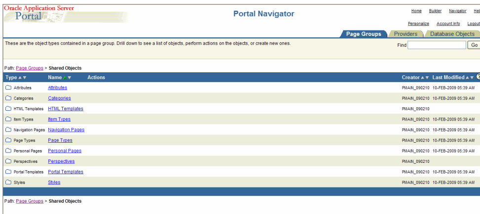
Figure 7-3 Shared Objects
