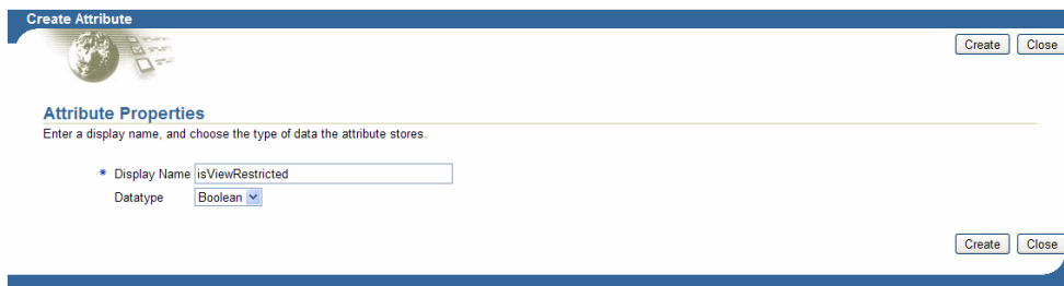
Figure 7-4 Create Attribute
